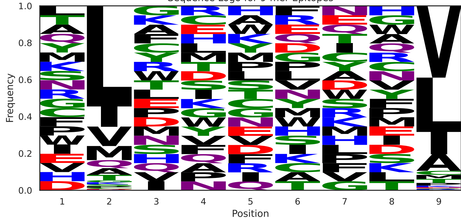
Sequence Logo for 9-mer Epitopes
