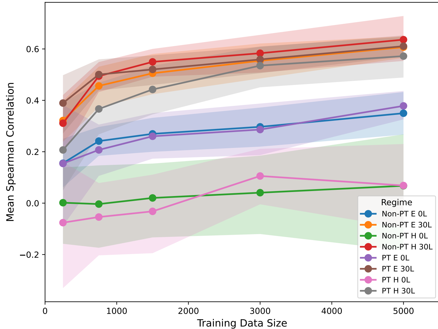
Performance vs Training Size
