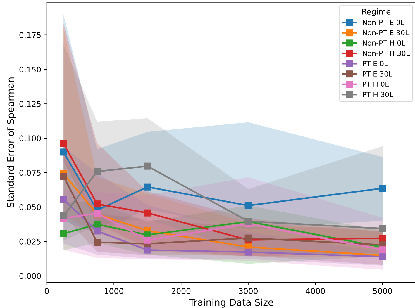
Stability vs Training Size
