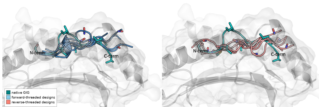
Figure 5: Forward vs. reverse threading, structural overlay (C18, 5 representative designs per panel, from a 186-design cohort). Native GIG peptide in teal (N-term/C-term labeled) against the MHC groove (white surface). Left panel: forward-threaded designs (sky blue) run N-to-C the same direction as the native peptide. Right panel: reverse-threaded designs (salmon) anchor the opposite end in the same F-pocket — the mirror-image backbone described in §3.4, made directly visible rather than inferred from a distribution.
