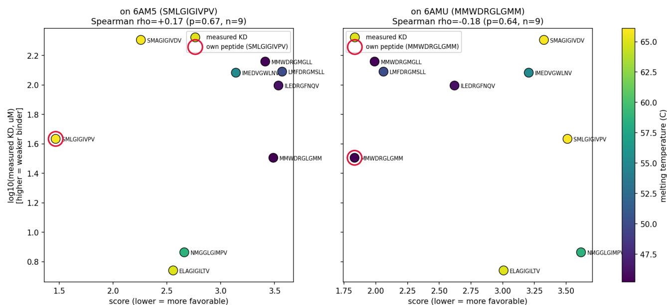
Figure S16: The score carries no information about measured affinity. LigandMPNN score against published K_D for the nine DMF5 peptides with an actual measured value, scored on 6AM5 (left) and 6AMU (right); points are colored by melting temperature and each structure's own crystallized peptide is circled. Four further peptides are excluded because their K_D is reported only as > 500 \mu\text{M} or as not detected, which is an assay ceiling rather than a measurement. Neither backbone shows a relationship. Contrast this with Figure 4, where the same scores separate the two peptide families cleanly: these models place a peptide, they do not rank it.
