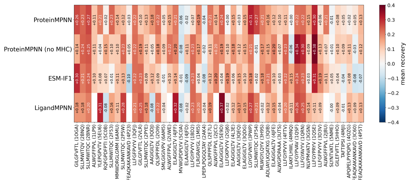
Figure 3: Where the TCR-context benefit actually concentrates. Recovery(full) – recovery(mhconly), per crystal per model, crystals ordered by resolution (best to worst, left to right).
