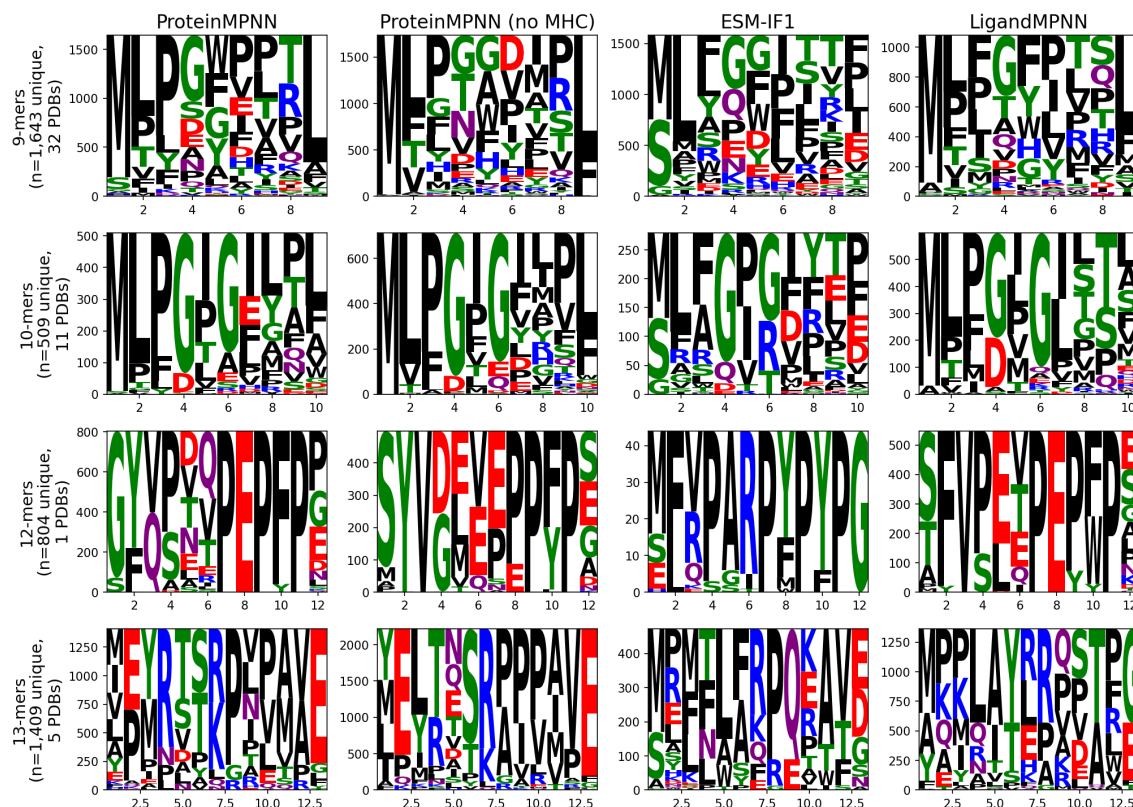
Figure S3: Design sequence logos, pooled by peptide length, one column per model.
