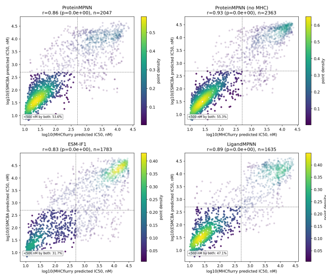
Figure 2: MHCflurry and ESM-CBA predictions of designs \log_{10}(\text{predicted IC}_{50}, \text{nM}) with pMHC+TCR context, one panel per model. Dashed lines mark the 500 nM; The percentage is the fraction of designs under 500 nM by both predictors at once.
