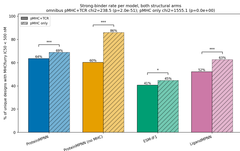
Figure S10: Removing the TCR raises predicted affinity for every model, by very different amounts. Strong-binder rate (MHCflurry IC 50 < 500 nM) per model in both structural arms; solid bars are pMHC+TCR, hatched bars pMHC only. Brackets give a Fisher's exact test of that model's own shift between arms, Bonferroni-corrected across the four models. Every model shifts up significantly, but the magnitude separates them: ProteinMPNN (no MHC) gains 25.7 percentage points and LigandMPNN 10.5, against 5.3 for ProteinMPNN and 4.0 for ESM-IF1. ESM-IF1 is the lowest-affinity model in both arms. The model ranking is preserved between arms, so the omnibus difference between models (reported above each arm) is not an artifact of which context is used.
