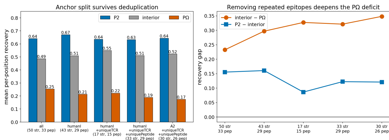
Figure S17: The anchor split is not an artefact of the panel's redundancy. The panel holds 50 structures but only 33 distinct peptides and 26 distinct CDR3 \beta sequences, so a pooled statistic weights an epitope by how often it was crystallised. Left, P2, interior and PΩ recovery on progressively stricter sets: human MHC class I only, then one structure per TCR family (CDR3 \beta clustered so clonotypes differing by one or two substitutions collapse), then one per peptide, then restricted to HLA-A*02:01; each group is represented by its best-resolution member, chosen independently of any score. Right, the same result as the two gaps that define it. Both survive, and the PΩ deficit deepens from 0.23 to 0.35 as repeated epitopes are removed. The one exception is P2 on the TCR-only set, which at 17 structures is underpowered rather than contradictory.
