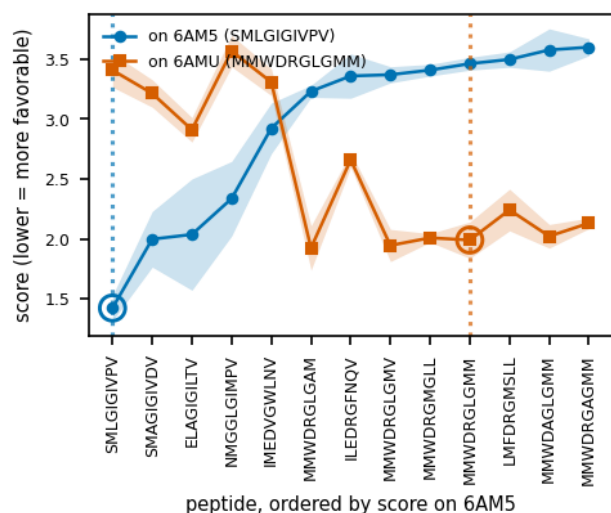
Figure 4: Each backbone favours its own crystallized peptide. The same 13 DMF5 peptides threaded onto 6AM5 (blue) and 6AMU (orange) and ordered by their score on 6AM5, shown as the mean of three models with a \pm 1 SD band, with rings and dotted lines marking each structure’s own peptide.
