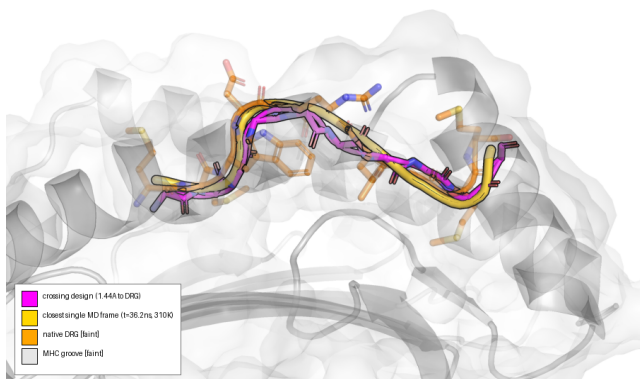
Figure 3: The closest crossing design against the single closest real MD snapshot. Magenta: the closest de-novo crossing design (6AM5_L3_nterm_t2, 1.44Å to the DRG register). Gold: the individual 310K/50ns MD frame it is nearest to ( t = 36.2 ns into the DRG trajectory, 1.03Å away) — an actual sampled thermal conformation, not the register’s time-averaged mean (orange, faint, shown for reference at 1.44Å). The two traces nearly coincide.
