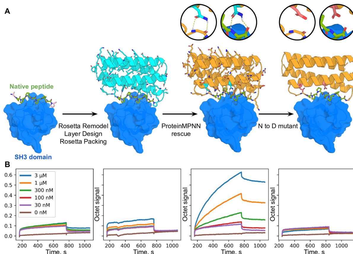
Fig. 4. Design of protein function with ProteinMPNN. (A) Design scheme. First panel; structure (PDB 2W0Z) of the peptide APPPRPPKP bound to the human Grb2 C-term SH3 domain (peptide is in green, target in surface and colored blue). Second panel: helical bundle scaffolds were docked to the exposed face of the peptide using RIFDOCK (19), and Rosetta remodel was used to build loops connecting the peptide to the scaffolds. Rosetta sequence design with layer design task operations was used to optimize the sequence of the fusion (Cyan) for stability, rigidity of the peptide-helical bundle interface, and binding affinity for the Grb2 SH3 domain. Third panel; ProteinMPNN redesign (orange) of the designed binder sequence; hydrogen bonds involving asparagine sidechains between the peptide and base scaffold are shown in green and in the inset. Fourth panel; Mutation of the two asparagines to aspartates to disrupt the scaffolding of the target peptide. (B) Experimental characterization of binding using biolayer interferometry. Biotinylated C-term SH3 domain from human Grb2 was loaded onto Streptavidin (SA) Biosensors, which were then immersed in solutions containing varying concentrations of the target peptide (left) of the designs (right panels), and then transferred to buffer lacking added protein for dissociation
