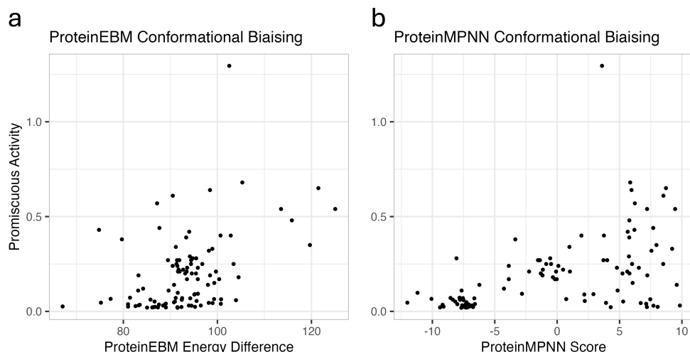
Figure S6: ProteinEBM-x can be applied to design conformationally biasing mutations. Correlation with LplA promiscuity for a.) ProteinEBM-x energy difference, b.) ProteinMPNN score.
