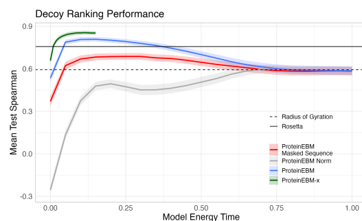
Figure S1: Rosetta test set spearman vs model energy time, including taking the norm of the score as a pseudo-energy.
