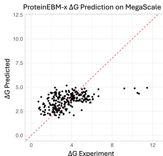
Figure S4: Evaluation of ProteinEBM-x \Delta G prediction on MegaScale dataset.
