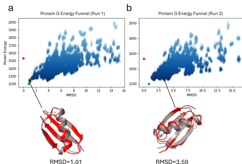
Figure S2: Two independent Langevin annealing runs, each with 400 trajectories. In a.) the lowest-energy sample adopts the correct fold and is extremely close to the native structure, while in b.) the lowest-energy sample has a swapped pair of strands compared to the native.
