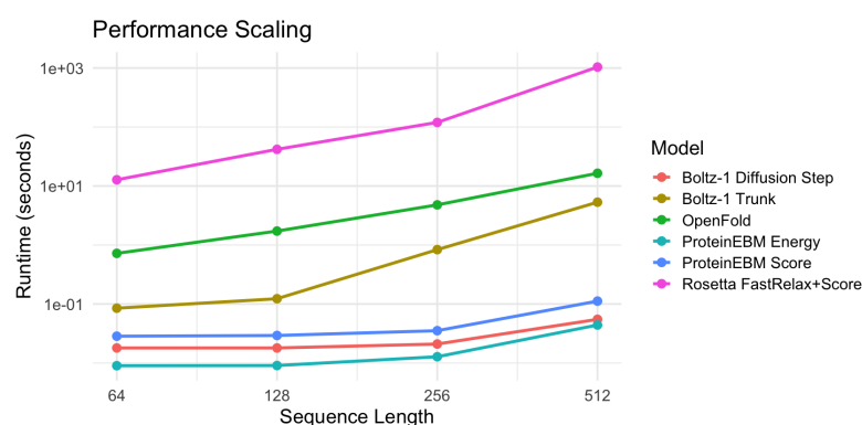
Figure S7: Runtime vs protein size for various protein modeling tools.
