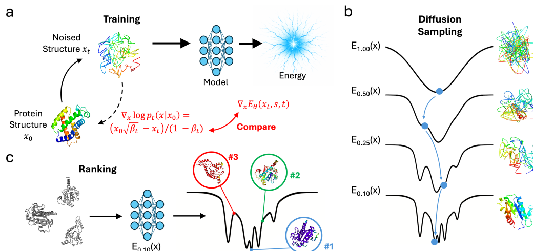
Figure 1: Overview of ProteinEBM. a.) Schematic of the score matching training process. b.) ProteinEBM can generate samples via reverse diffusion over the learned energy landscapes. c.) ProteinEBM can rank arbitrary input structures via its learned energy.
