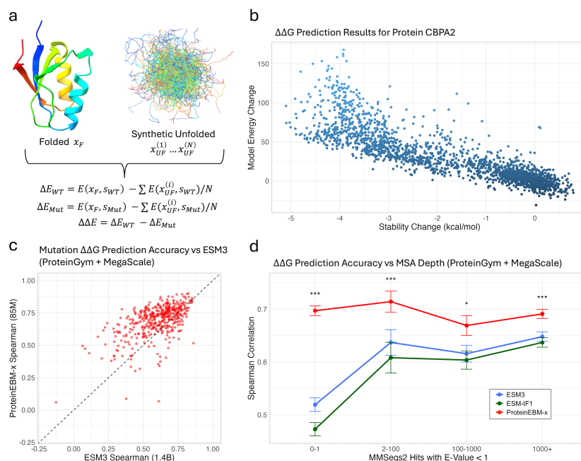
Figure 3: ProteinEBM-x energies accurately predict changes in protein stability. a.) Method for approximating \Delta\Delta G with folded and unfolded structures b.) Example correlation between predicted and experimental \Delta\Delta G for protein CBPA2. c.) Spearman correlations between ProteinEBM-x energy differences and experimental \Delta\Delta G s vs ESM3 Spearman for all stability targets in ProteinGym and MegaScale c.) ProteinEBM-x, ESM3, and ESM-IF1 Spearman on ProteinGym and MegaScale v.s. the MSA depth of each protein. Error bars are standard error of the mean.
