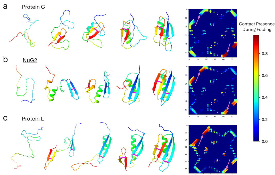
Figure 5: ProteinEBM-x can be used to rapidly simulate folding trajectories of proteins. a.) Left: An example folding trajectory for Protein G, with snapshots taken at different frames from the simulation. Formation of example contacts labeled in Magenta. Right: Contact presence fraction during folding transitions, with example contacts indicated with magenta arrows. b.) Same as part a for NuG2. c.) Same as part a for Protein L.
