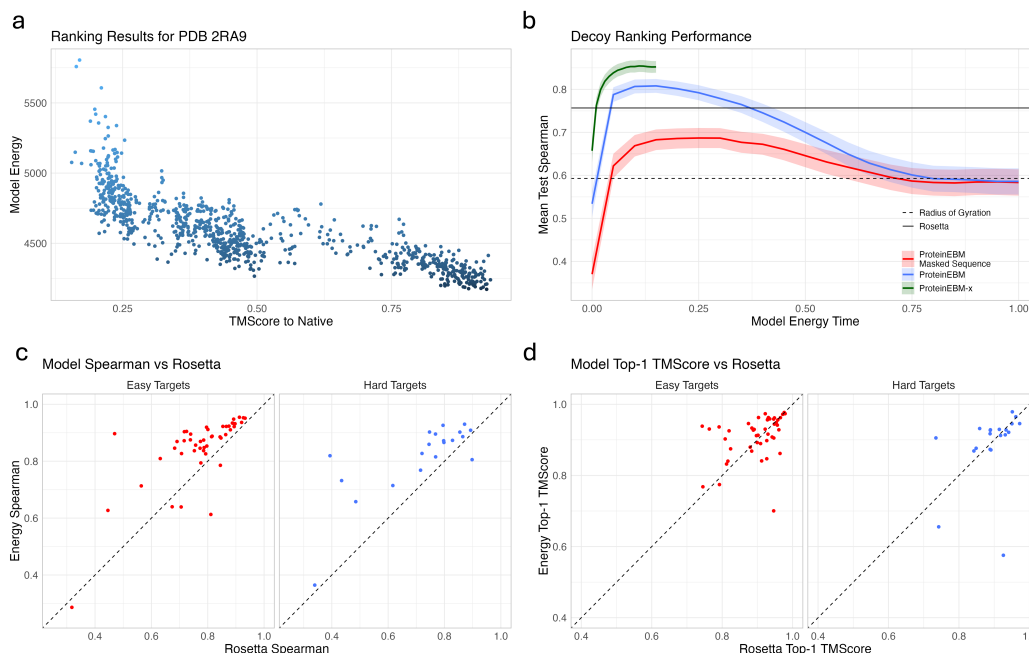
Figure 2: ProteinEBM-x can be used to accurately rank protein structure accuracy. a.) Example correlation between ProteinEBM-x energy and decoy TMScore for a test set protein. b.) Mean Spearman correlations between energy and TMScore at different values of t . Ribbons are standard error of the mean. c.) Comparison of Spearman correlations for ProteinEBM-x and Rosetta on each target in the test set. Dots are separated into easy and hard targets. Hard targets were subjected to a structure-based split and are farther from the training set d.) Comparison of the TMScore of the top-ranked decoy for each test target for ProteinEBM-x and Rosetta.
