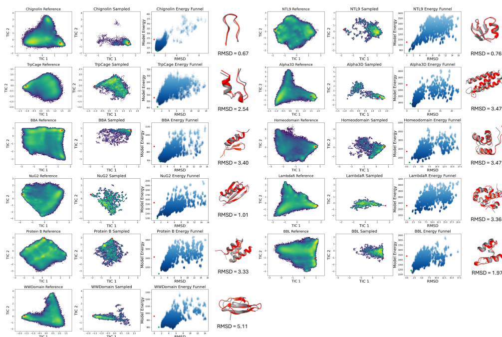
Figure 4: ProteinEBM effectively samples conformations of fast-folding proteins with Langevin annealing. TICA plots showing conformational landscape for MD simulations (left) and ProteinEBM samples (right) for each fast folder, with red dot indicating native structure. Energy funnels show the relationship between model energy ( t = .05 ) and RMSD to native for sampled structures. For funnel plots, the red dot indicates the native structure and green dot indicates the native after running a fast relaxation procedure. For protein structure graphics, the lowest-energy ProteinEBM sample is in red, and the native is in gray.
