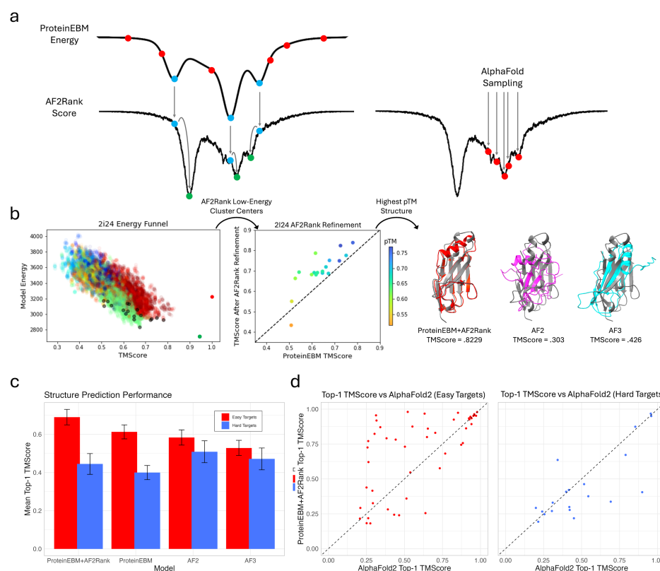
Figure 6: ProteinEBM and ProteinEBM-x can be used to sample and score structure predictions. a.) ProteinEBM Langevin annealing (left) explores broadly, and the best samples are passed to AF2Rank. Standard AlphaFold sampling (right) can fail to sample global minima. b.) Left: TMScore vs Energy for ProteinEBM samples on PDB 2i24. Red dot is native, green dot is relaxed native, colors are clusters, gray dots are cluster centers. Center: AF2Rank refines and reranks lowest-energy cluster centers. Right: Predicted vs native structure for ProteinEBM+AF2Rank, AF2, and AF3. c.) Average top-1 TMScore for ProteinEBM, ProteinEBM+AF2Rank, AF2 and AF3, with performance split between easy and hard targets. Error bars are standard error of the mean. d.) Scatter plot of top-1 TMScores for ProteinEBM+AF2Rank vs AF2, split by easy and hard targets.
