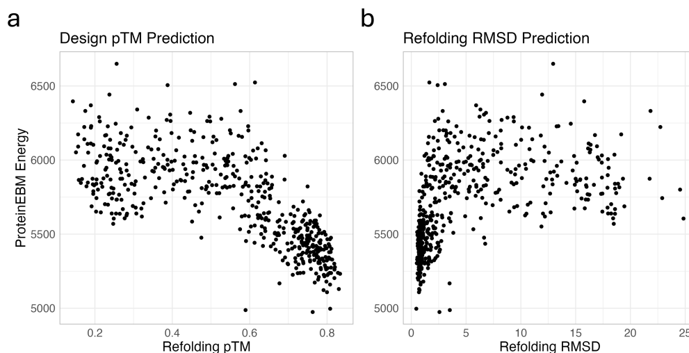
Figure S5: ProteinEBM-x can be used to filter designed proteins. a.) Correlation between ProteinEBM energy of design and Boltz-2 refolding pTM b.) Correlation between ProteinEBM energy of design and Boltz-2 refolding RMSD.
