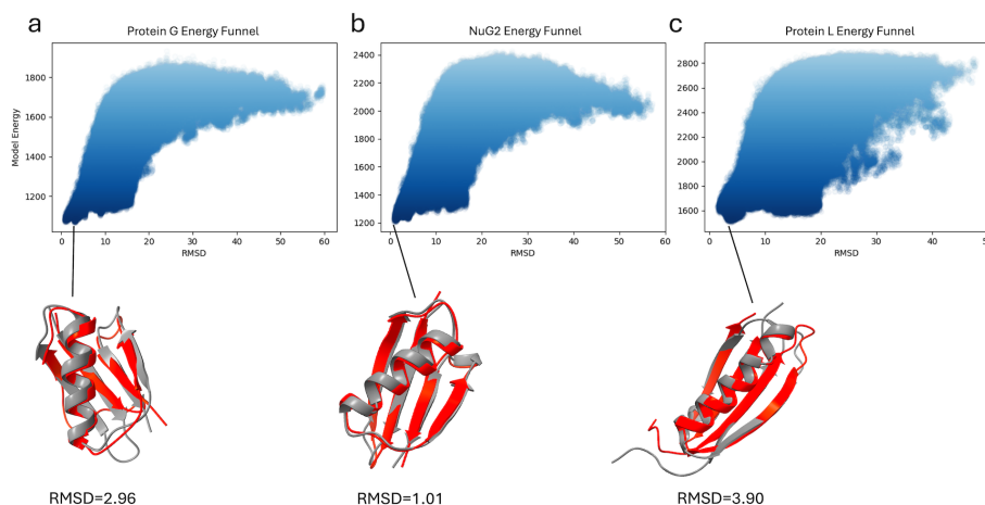
Figure S3: Energy funnels for direct folding simulations for a.) Protein G, b.) NuG2, and c.) Protein L. The lowest-energy samples for Protein G and NuG2 both have the same fold as the native, while for Protein L the lowest-energy structure has a swapped pair of strands.
