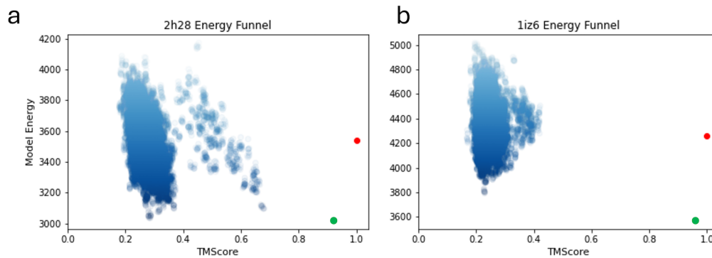
Figure S9: Energy funnels for failed prediction targets, with native structure as red dot and relaxed native structure as green dot. a.) Example where ProteinEBM explored a structure close to the native (TMScore \approx 0.7 ), but erroneously scored a much less accurate structure with lower energy. b.) Example where the model failed to explore close to the native structure, although the native structure had a far lower energy than the structures that were actually sampled.
