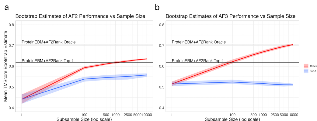
Figure S8: Examining the effect of sample size on AF2 and AF3 structure prediction. a.) Oracle TMScore and TMScore of top-ranked decoy for AF2 as number of samples is increased. b.) Oracle TMScore and TMScore of top-ranked decoy for AF3 as number of samples is increased. Ribbons are 95% bootstrap confidence intervals of the mean.
