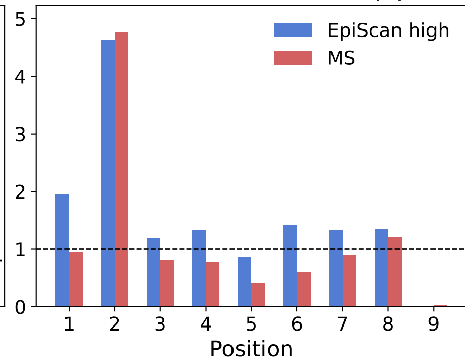
Enrichment for Serine (S)
