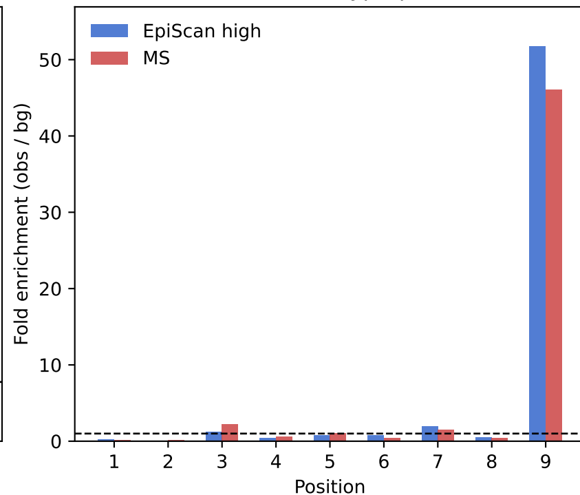
HLA-B5701 Enrichment (9-mers) Enrichment for Tryptophan (W)
