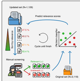
Mode 3: AIM Review screening with active learning
