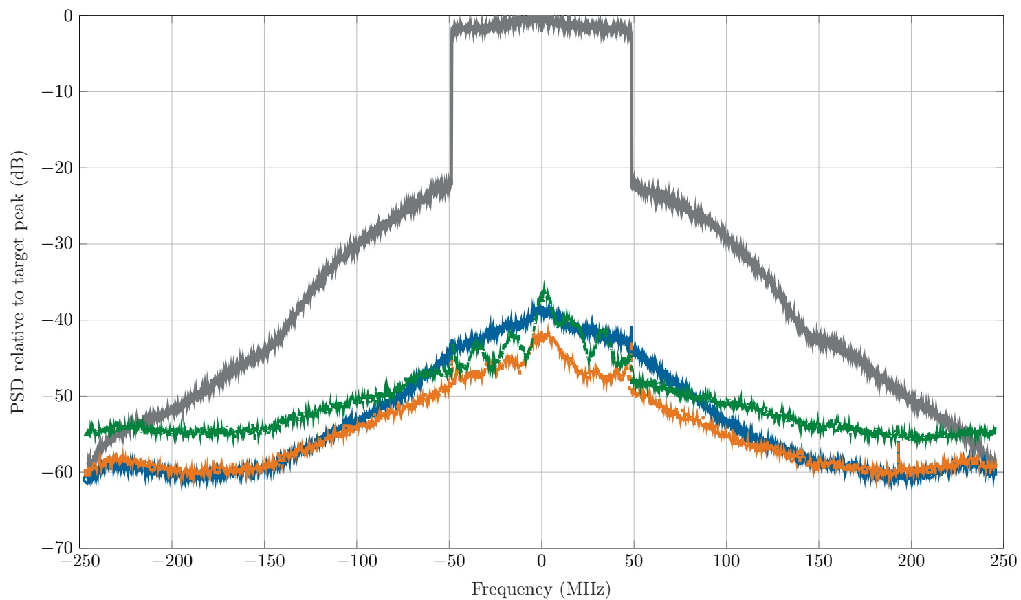
— Target full signal — Complex GMP-DOMP error — PN-IQ PN-DOMP error — Sparse PNNN N12 error
