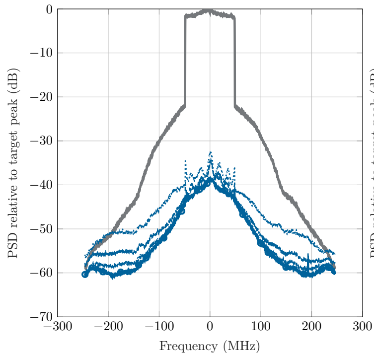
(a) Complex GMP-DOMP
