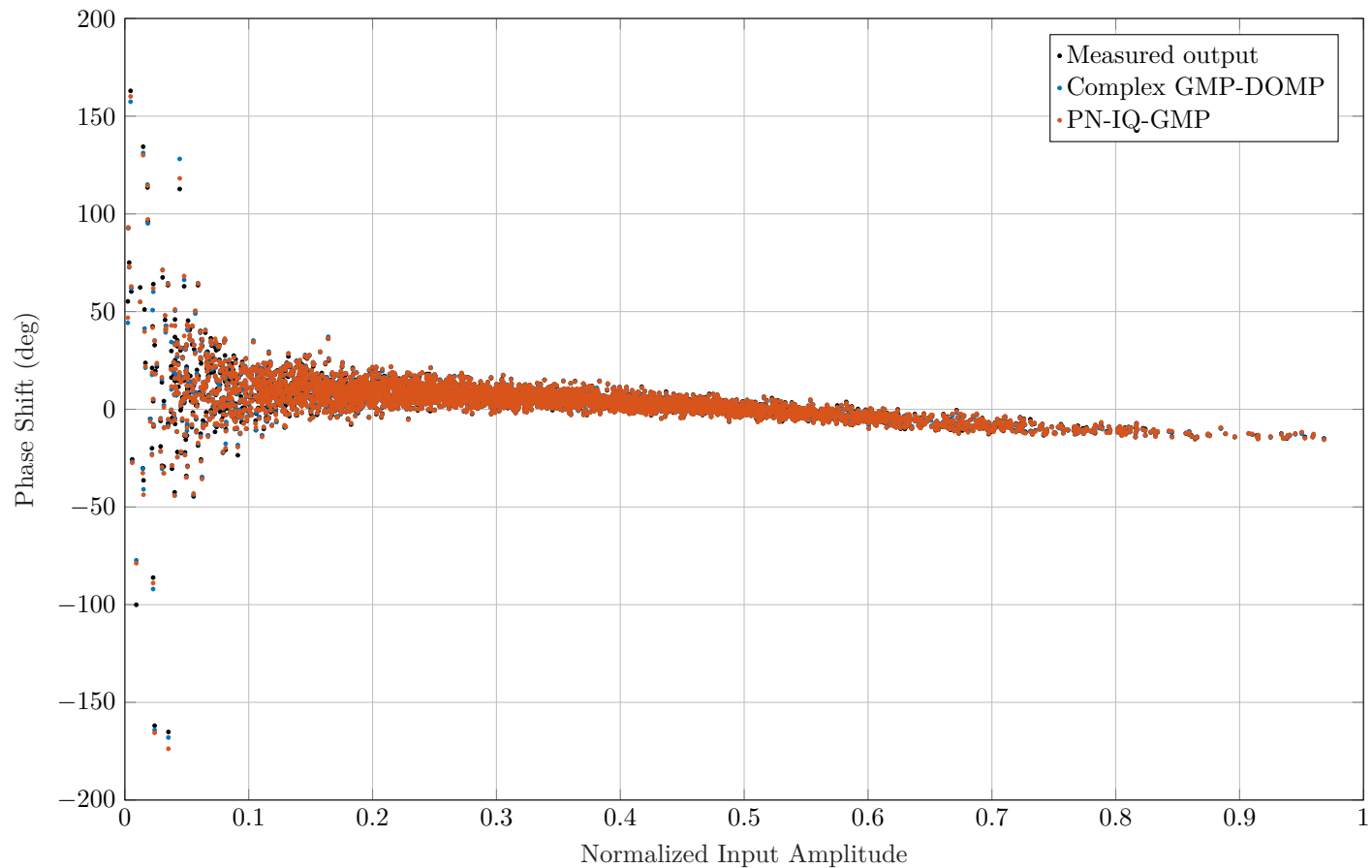
Measured and Modeled AM/PM Characteristics
