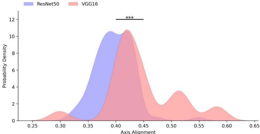
Figure 5: Axis-alignment as a proxy measure of superposition. We measure the axis-alignment of dictionary elements recovered by CRAFT for both models using the sparsity measure of Hoyer (2004) (see Eq. 2). Higher values indicate stronger alignment with individual neuron axes, i.e. , the recovered dictionary elements can be well approximated by single neurons. We find that ResNet50 has significantly lower axis-alignment than VGG16: 0.40 vs. 0.45, z = 6.01 , p < .001 (Mann–Whitney U test). This suggests that ResNet50 is more impacted by superposition.
