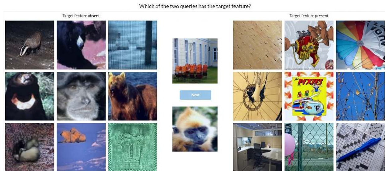
Figure A1: Illustration of the role of semantics. Example of a trial from Experiment I in the neuron-based representation condition. In this case, the task can be trivially solved by relying on semantic grouping. By observation of the minimally activating stimuli (left panel), it is easy to conclude that the neuron of interest is not a monkey detector, yet, it is hard to articulate what visual pattern is captured by the neuron (images in the right panel).
