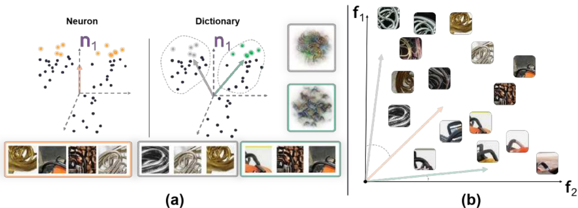
Figure 1: (a) • Neuron (axis) basis versus • Dictionary basis . Individual neurons may respond to multiple unrelated visual patterns (bottom), whereas dictionary learning aims to recover feature directions that isolate simpler patterns. (b) Dictionary learning yields a new basis over activations whose elements ideally correspond to single patterns. The interpretability hope is that these patterns align with the set of human-recognizable concepts S = \{f_1, f_2, \dots, f_n\} .
