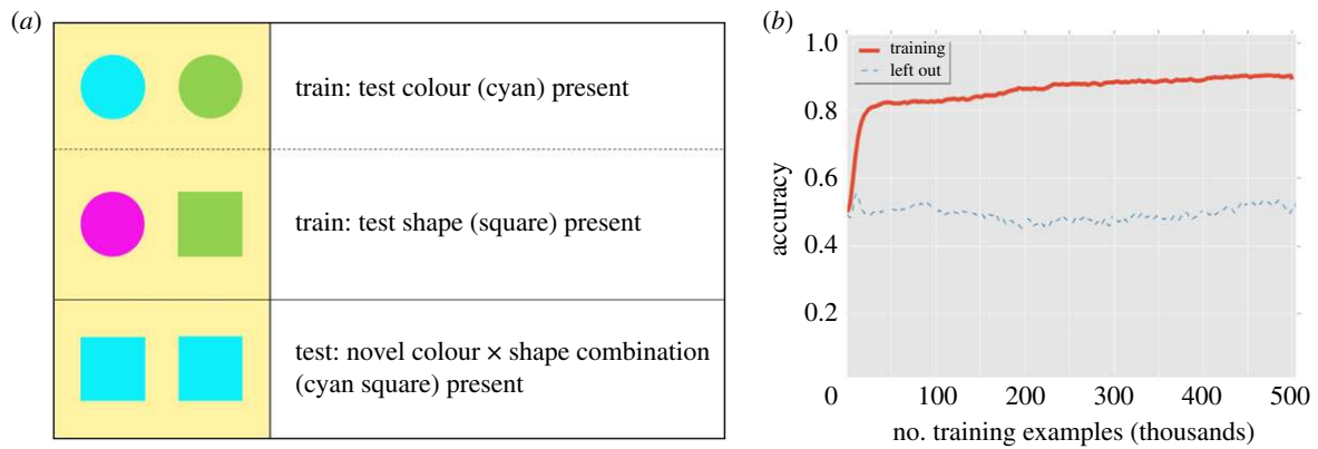
Figure 7. (a) Sample items used during training and testing in experiment 3. We trained relational networks (RNs) on 12 two-item same–different datasets each missing one colour–shape combination from sort-of-CLEVR (2 shapes \times 6 colours). Then, we tested the model on the left-out combination. The top and middle rows of panel (a) show two possible pairs of items when the left-out combination is ‘cyan square’. Row 1 shows a cyan circle and row 2 shows a green square. However, only in the test set is the model queried about images involving a cyan square (e.g. the ‘same’ image in row 3). Note that, during training, the model observes each left-out attribute, just not in the left-out combination. (b) Averaged accuracy curves of an RN while being trained on the sort-of-CLEVR datasets missing one colour–shape combination. The red curve shows the training accuracy. The blue dashed line shows the accuracy on validation data with the left-out items.
