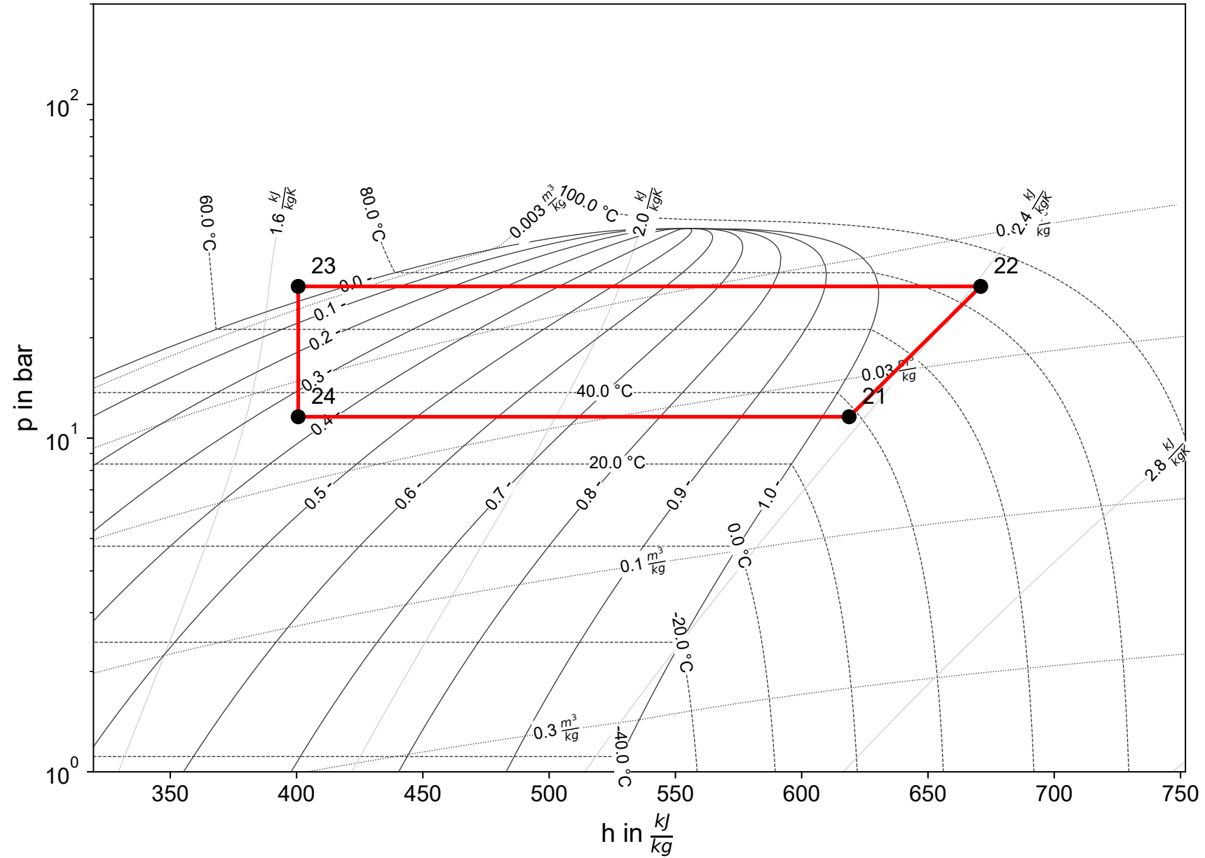
Cycle 1 (R290)
