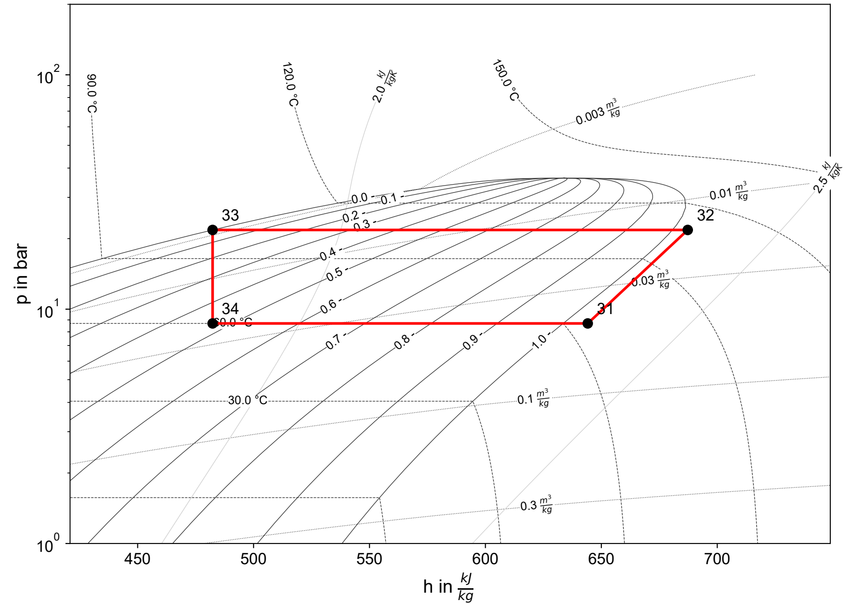
Cycle 2 (R600a)
