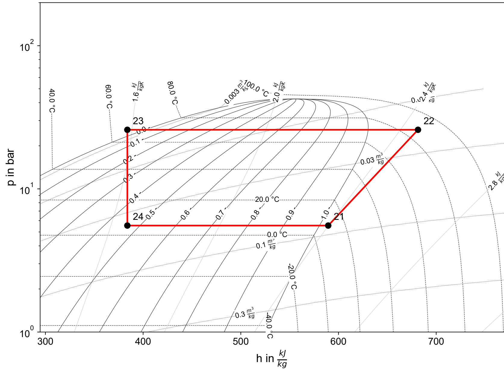
Cycle 1 (R290)
