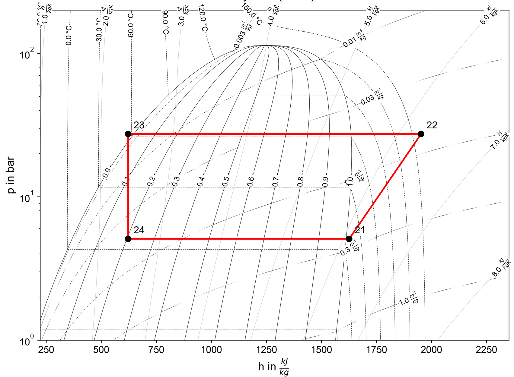
Cycle 1 (R717)
