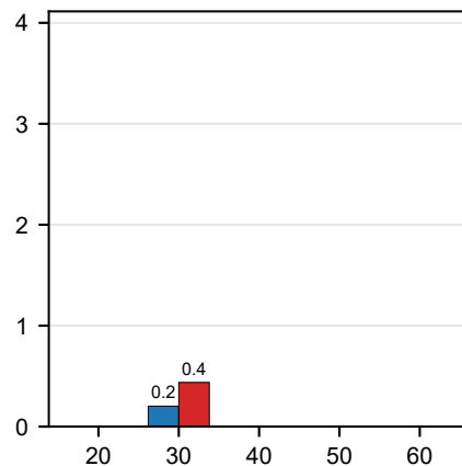
R717/R600a
