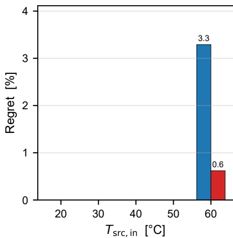
R290/R600a
