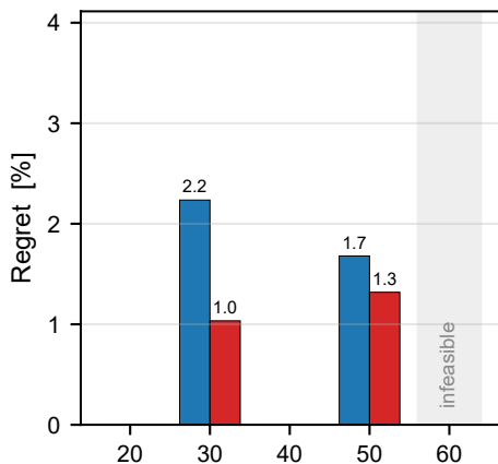
R290/R600a
