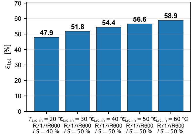
Exergetic efficiency
