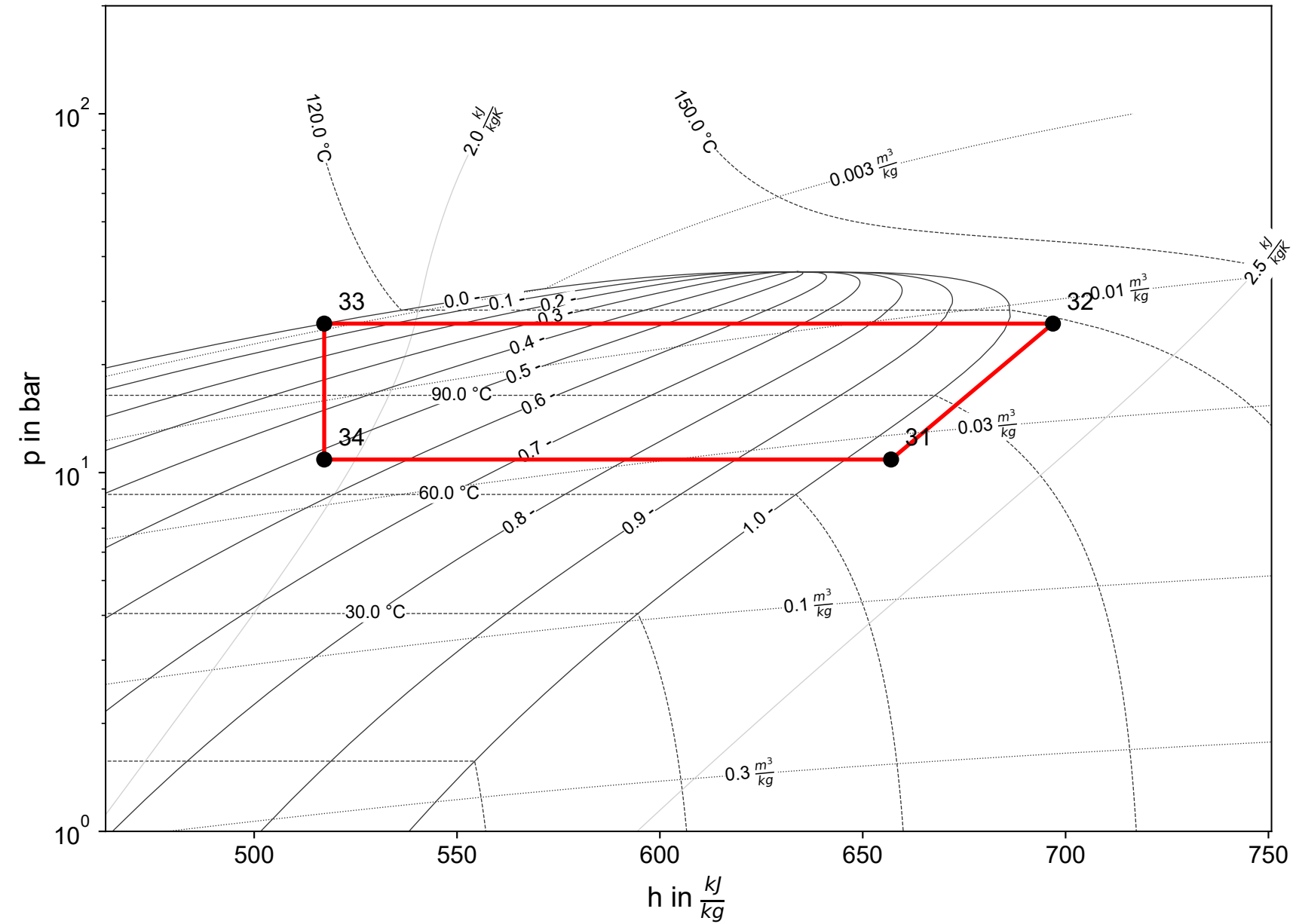
Cycle 2 (R600a)
