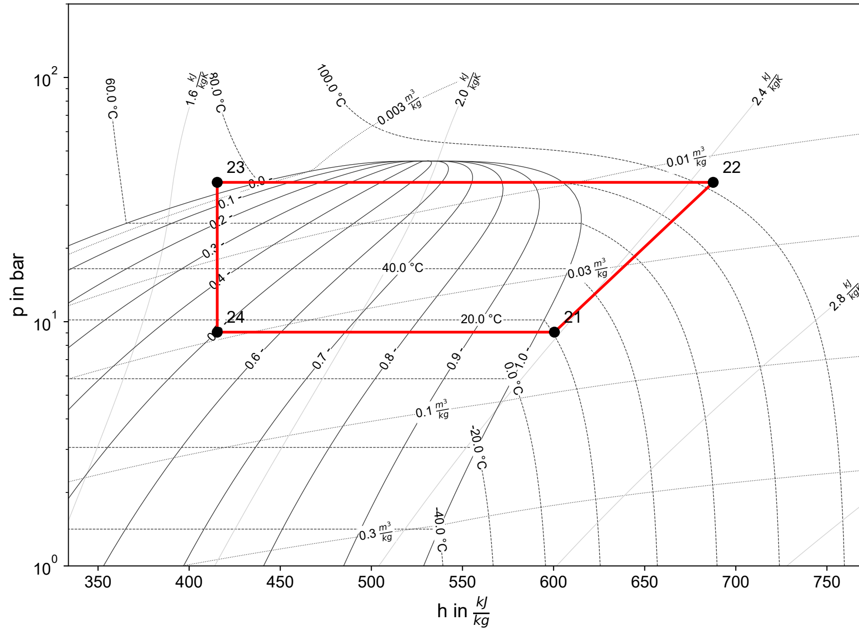
Cycle 1 (R1270)
