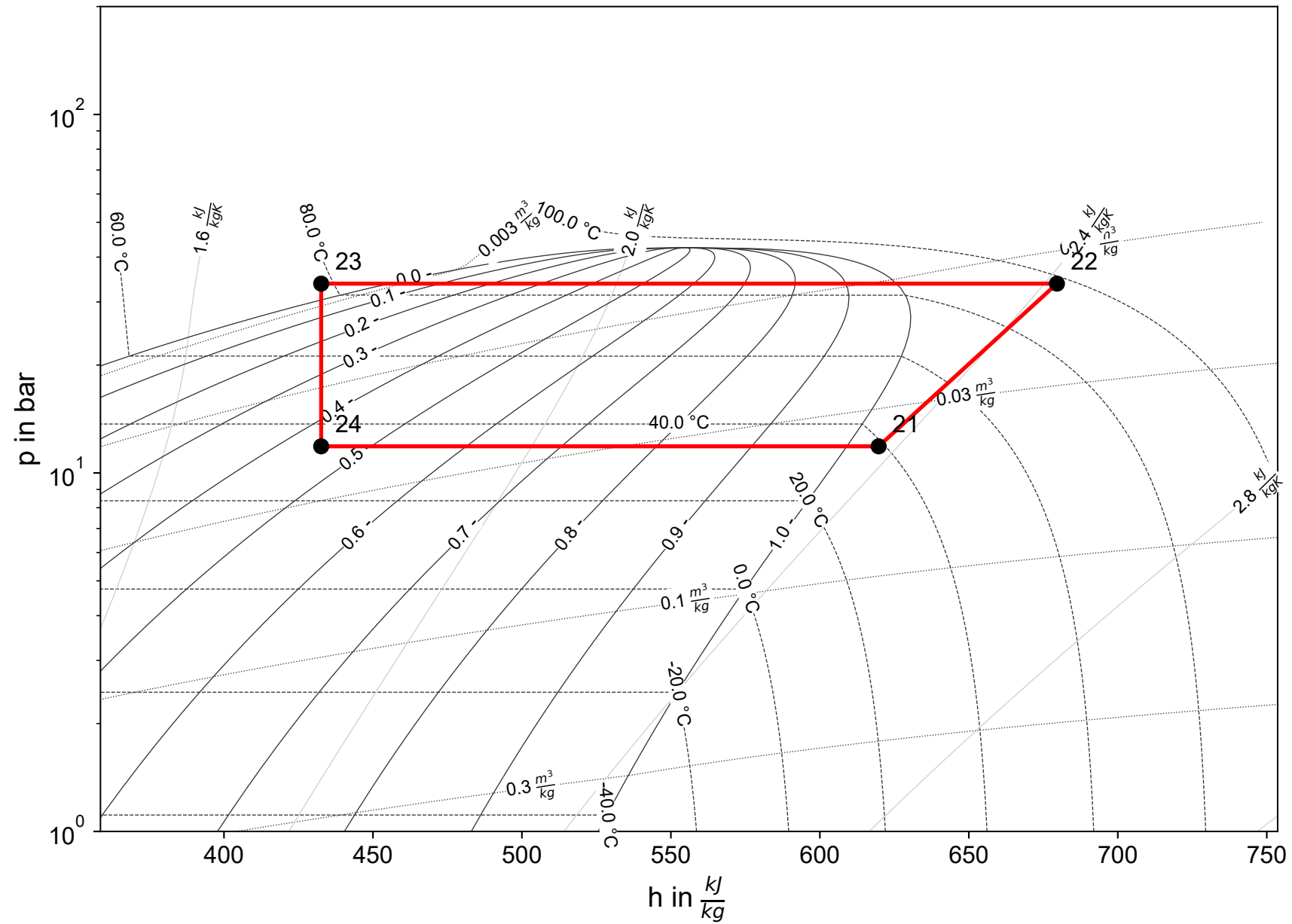
Cycle 1 (R290)
