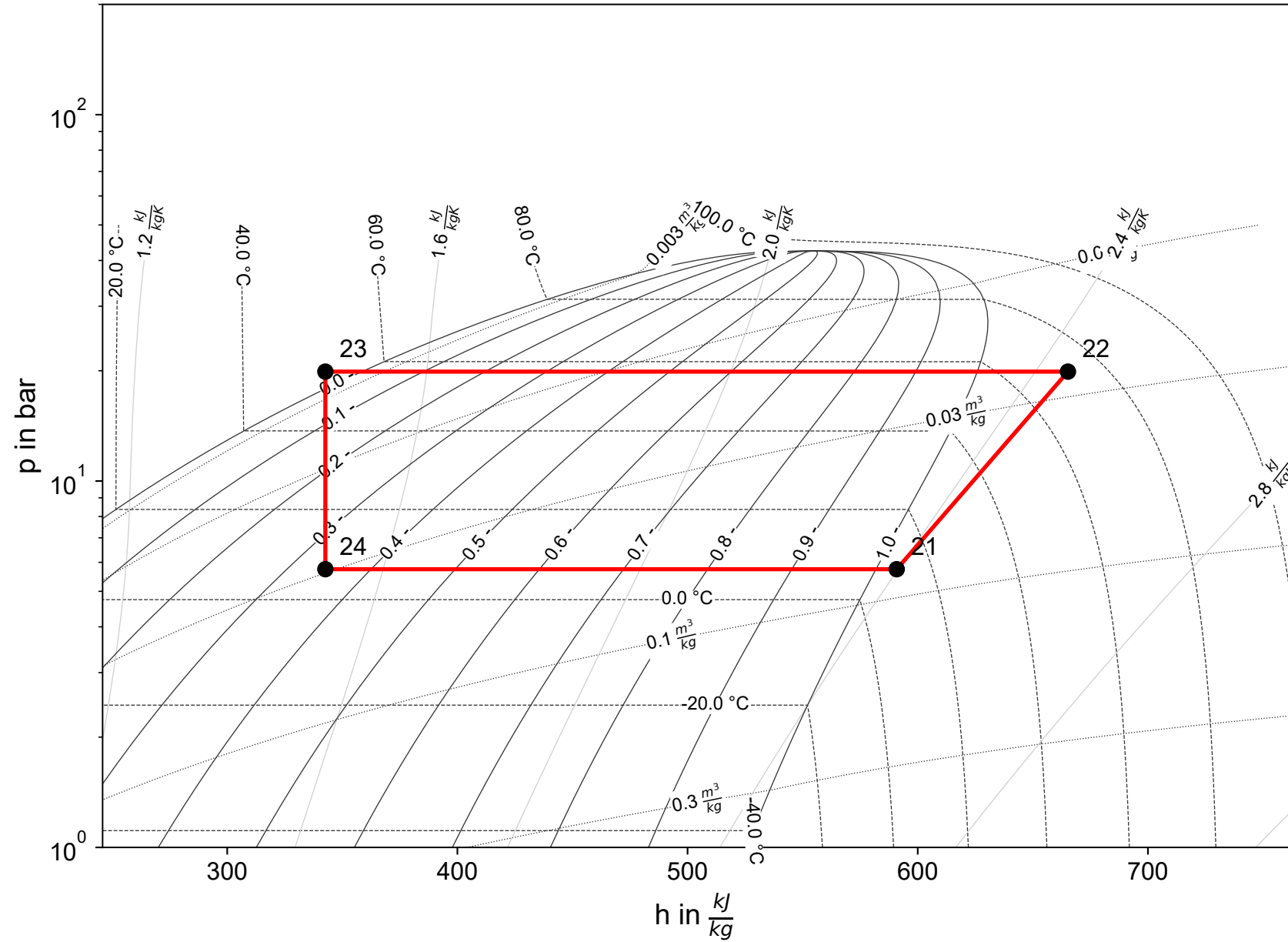
Cycle 1 (R290)
