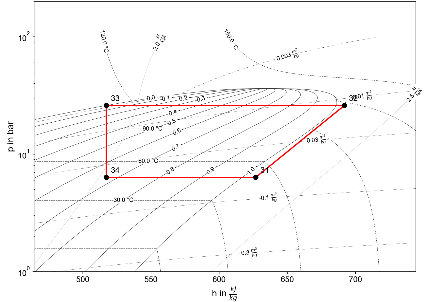
Cycle 2 (R600a)
