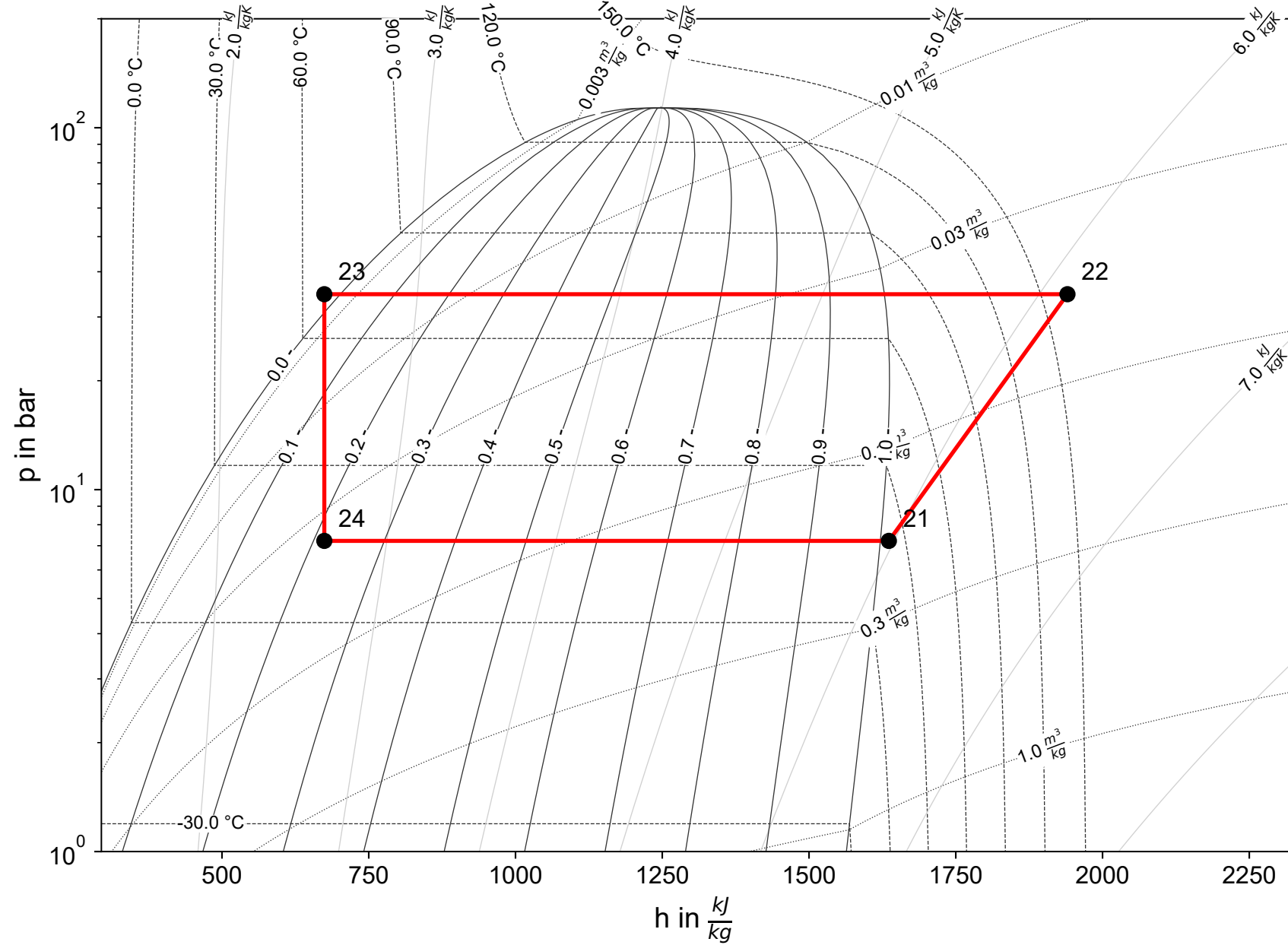
Cycle 1 (R717)
