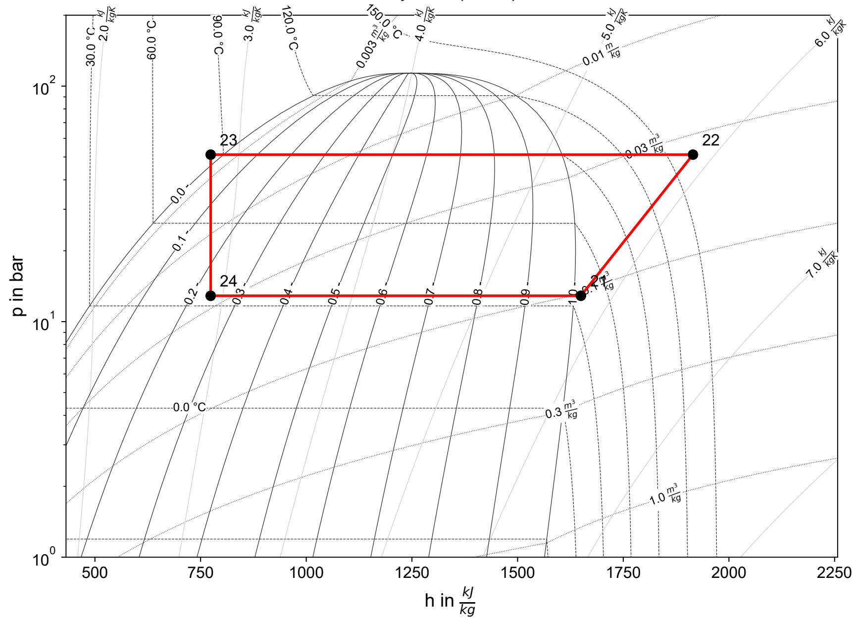
Cycle 1 (R717)
