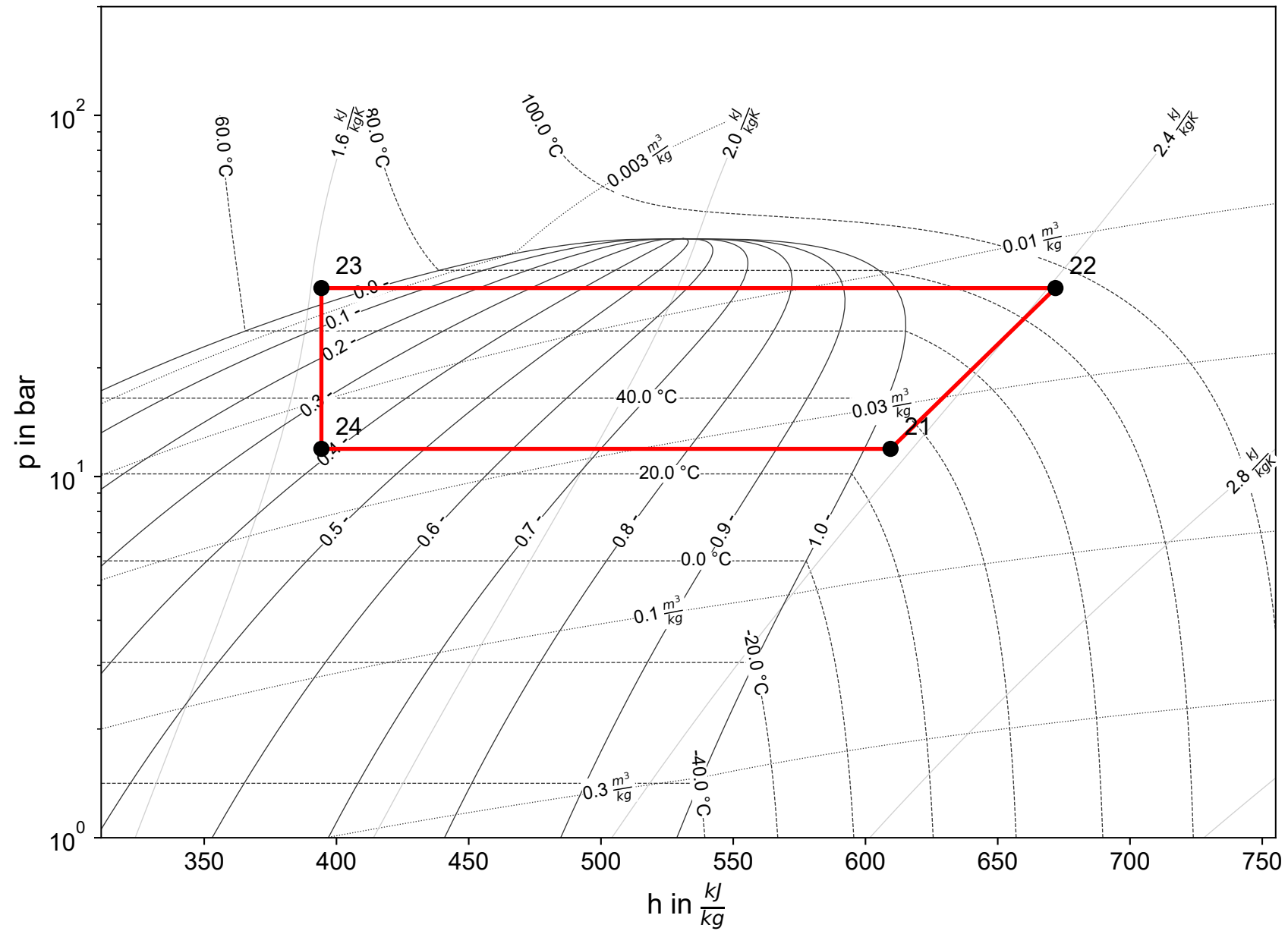
Cycle 1 (R1270)
