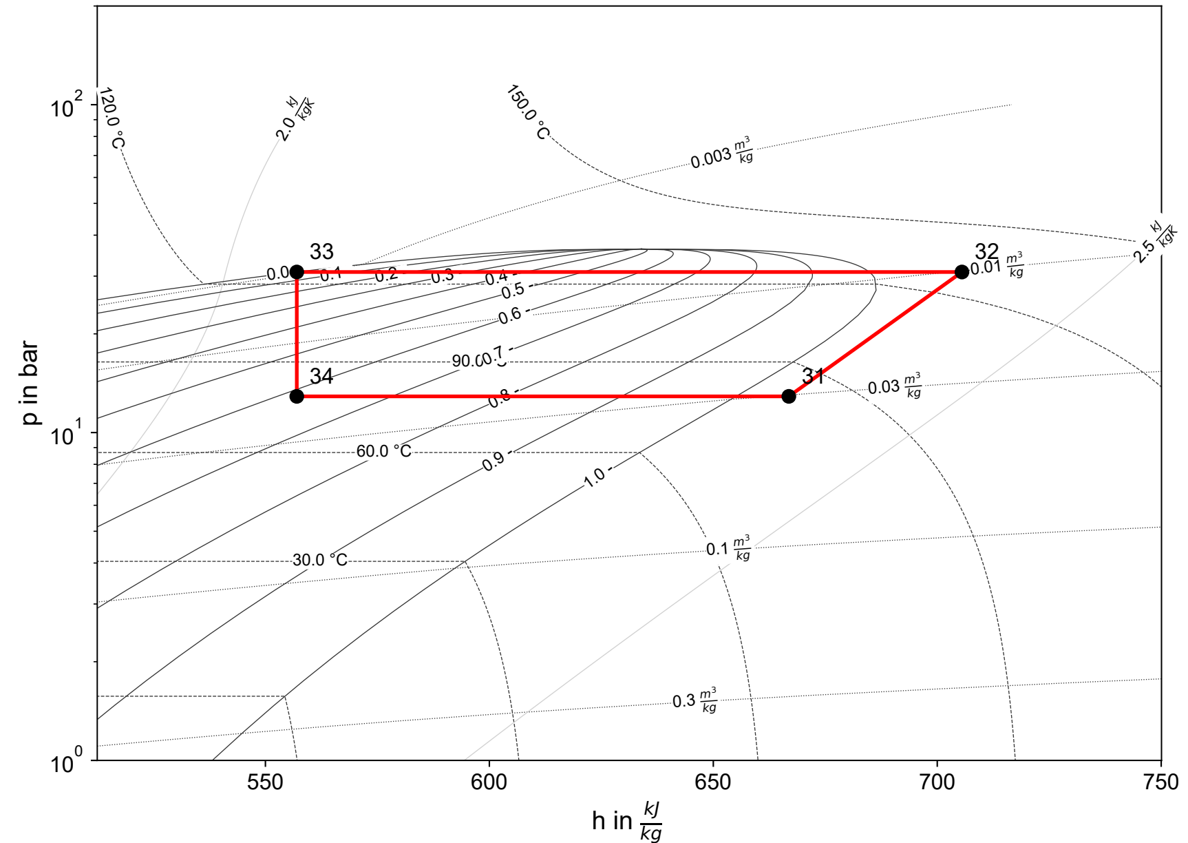
Cycle 2 (R600a)
