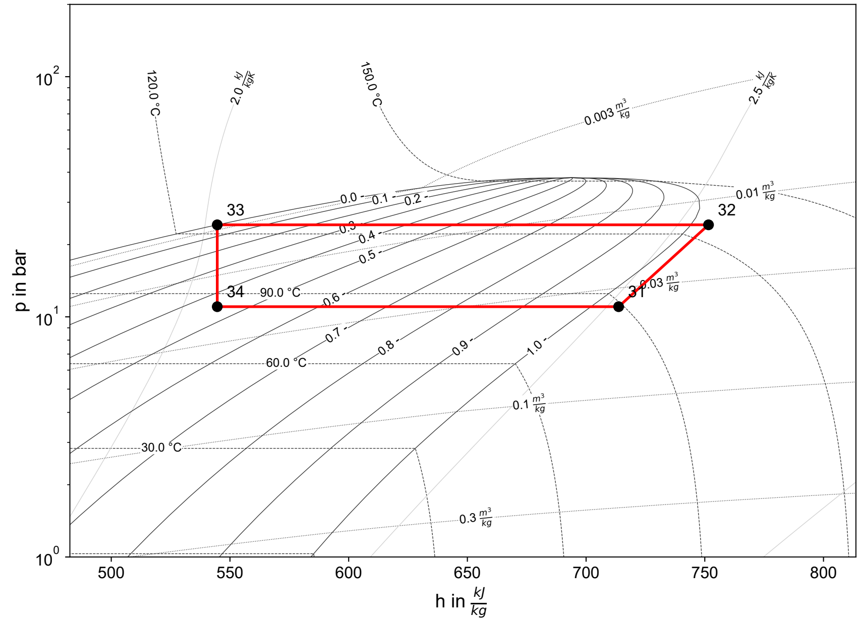
Cycle 2 (R600)
