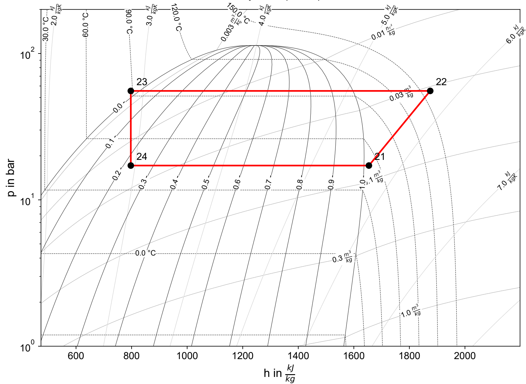
Cycle 1 (R717)
