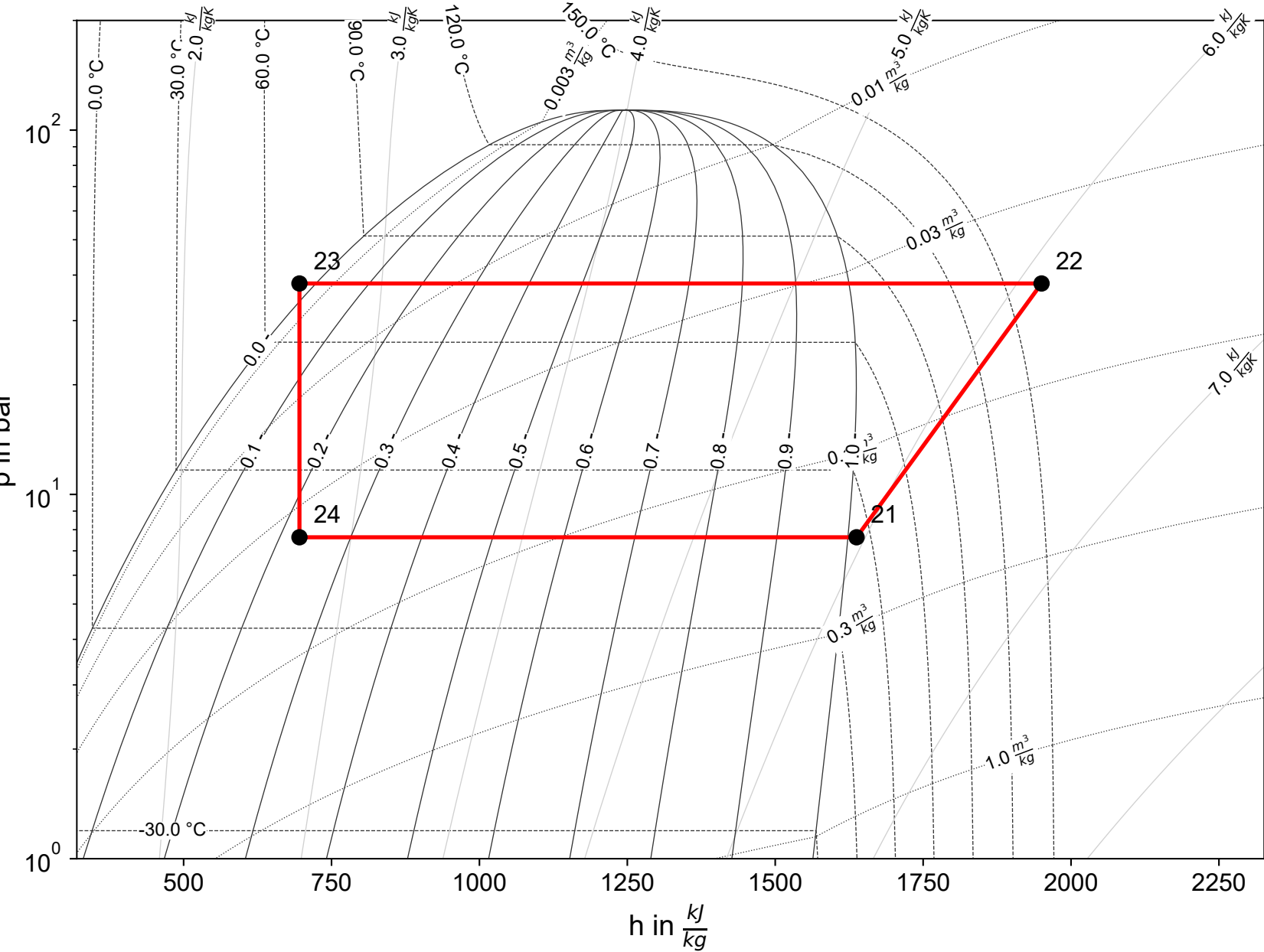
Cycle 1 (R717)
