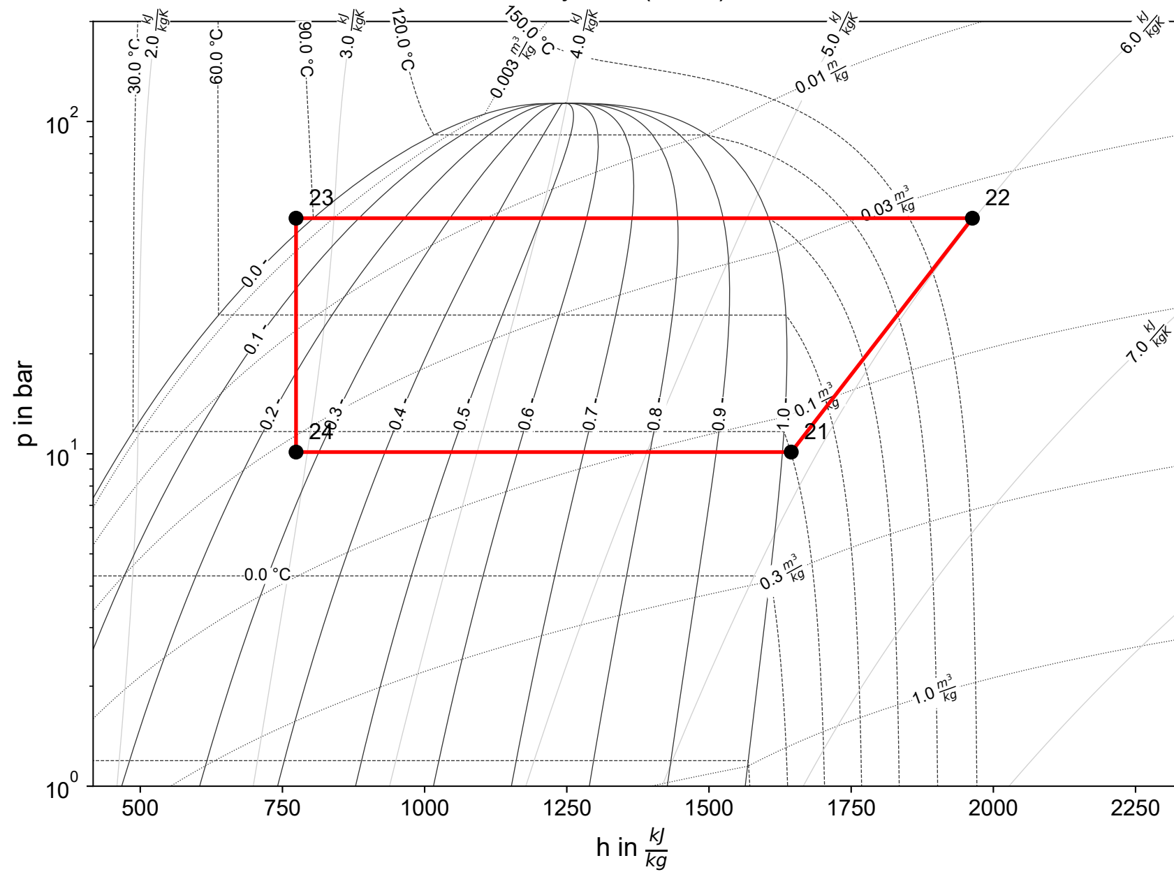
Cycle 1 (R717)
