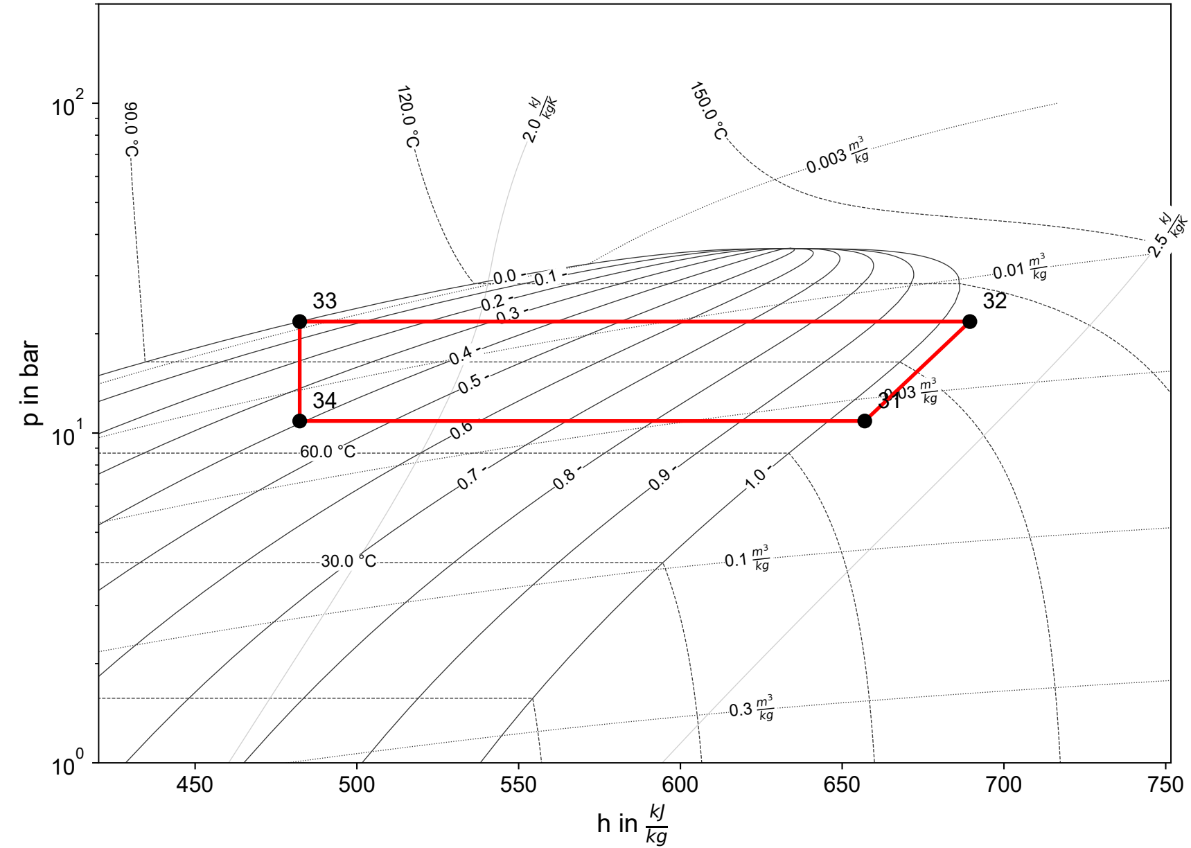
Cycle 2 (R600a)
