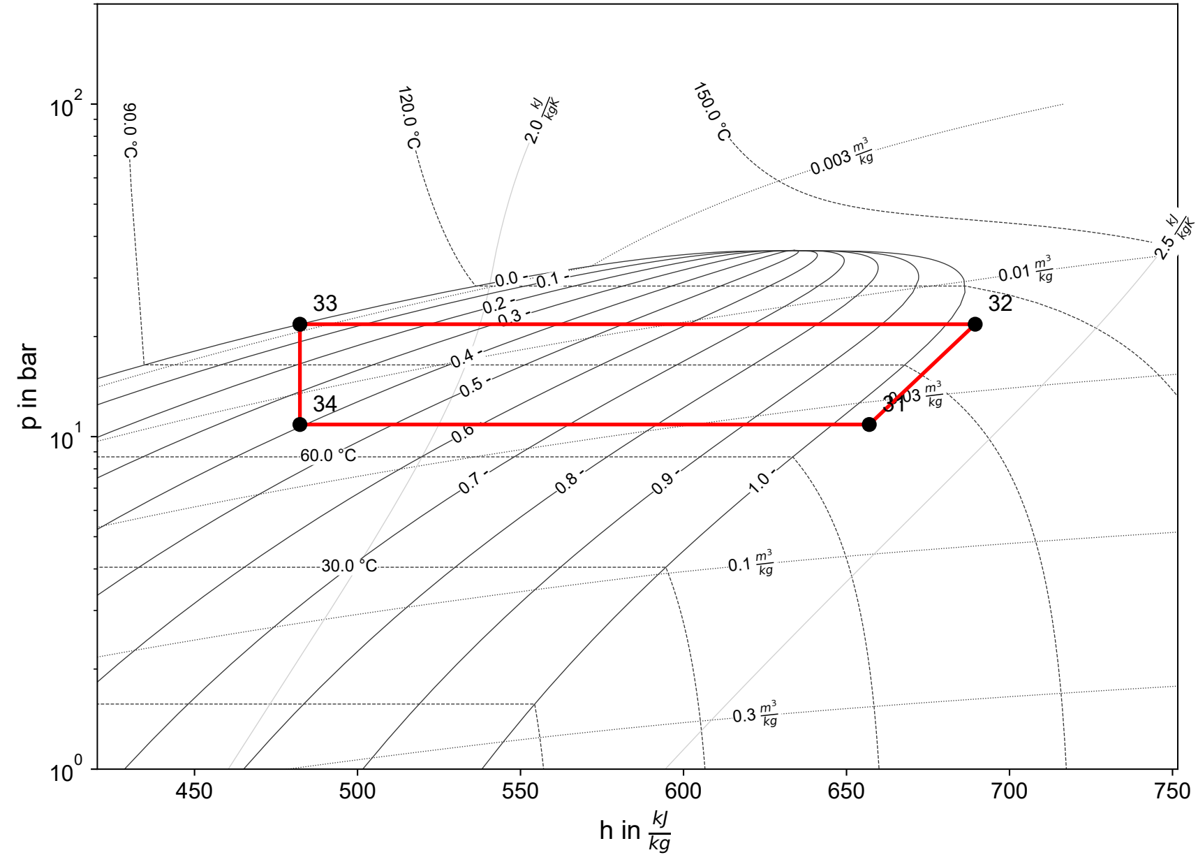
Cycle 2 (R600a)
