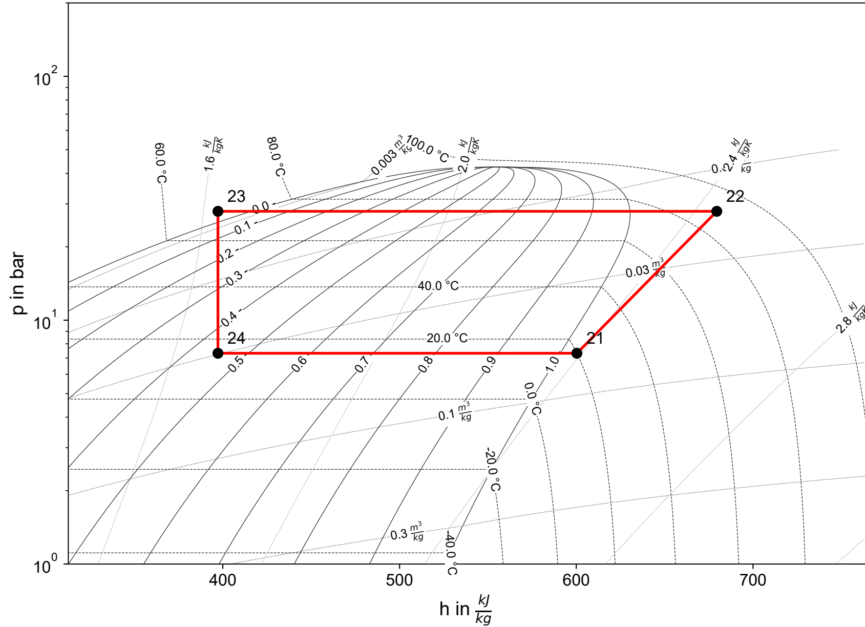
Cycle 1 (R290)
