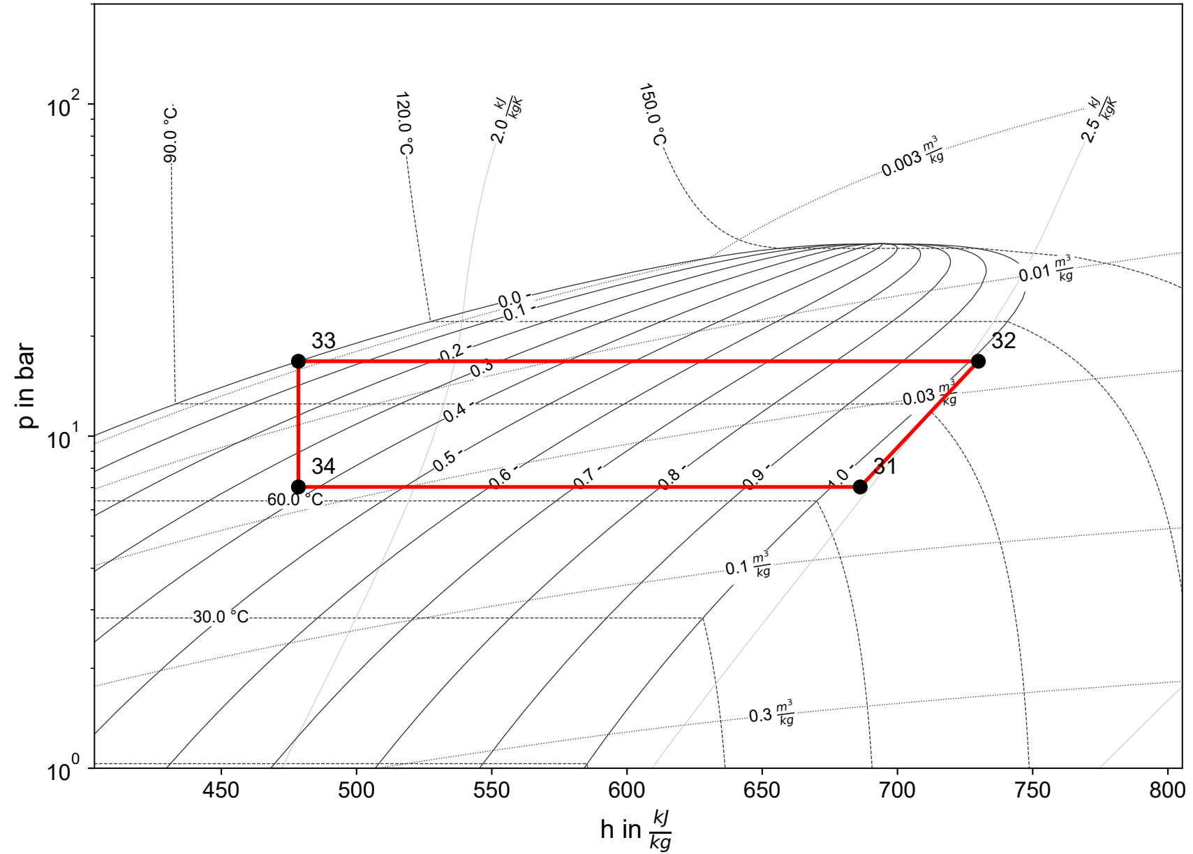
Cycle 2 (R600)
