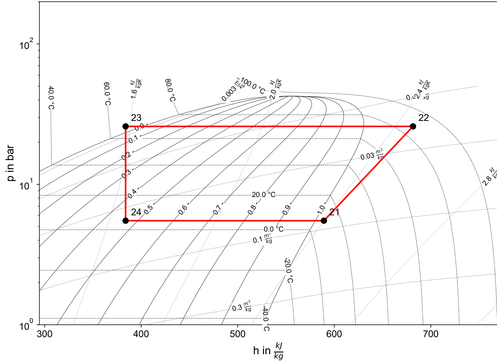
Cycle 1 (R290)
