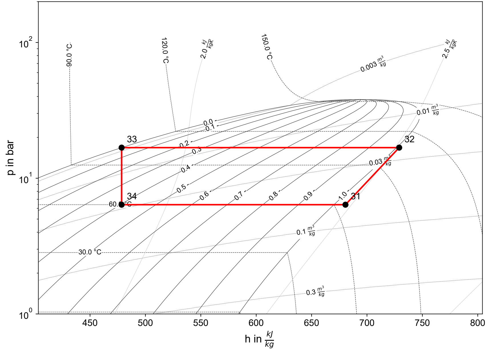
Cycle 2 (R600)
