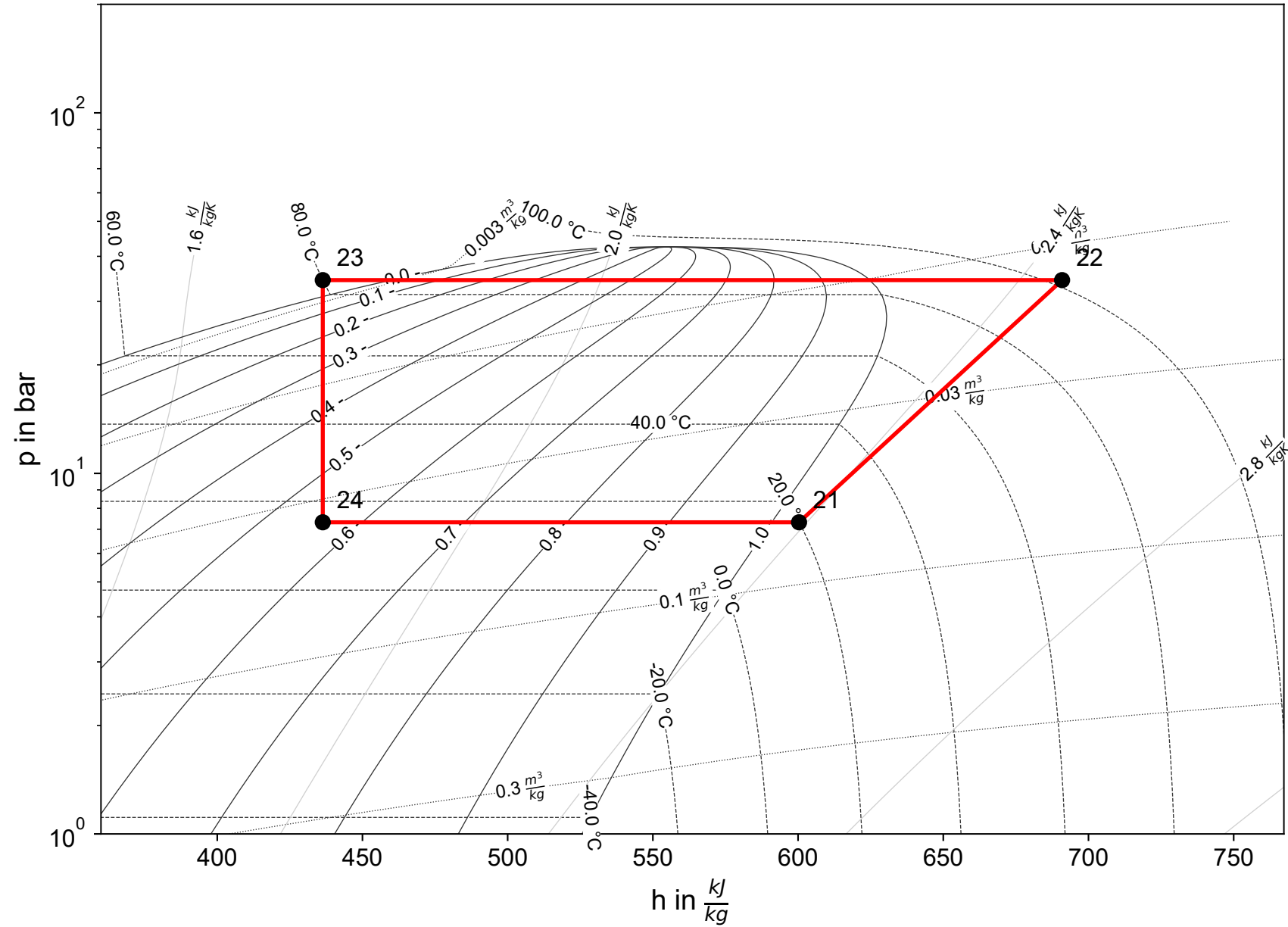
Cycle 1 (R290)
