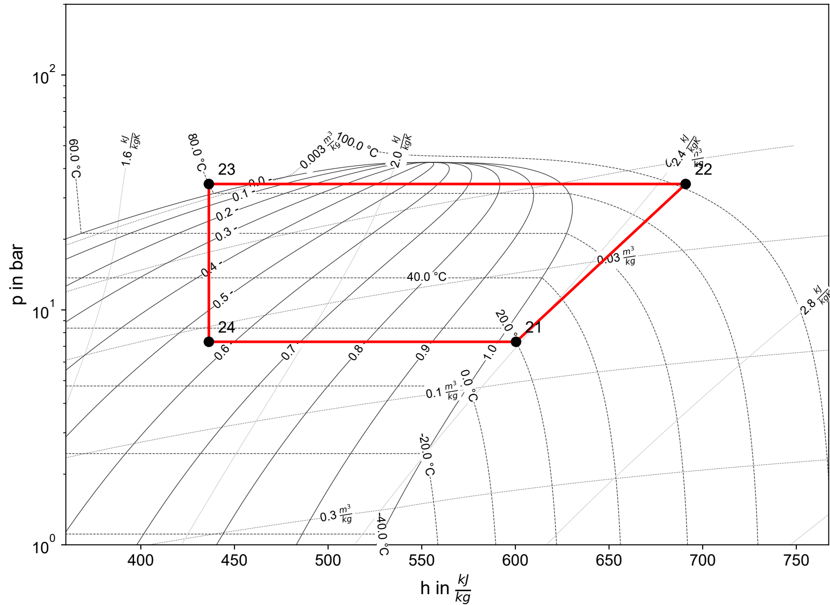
Cycle 1 (R290)
