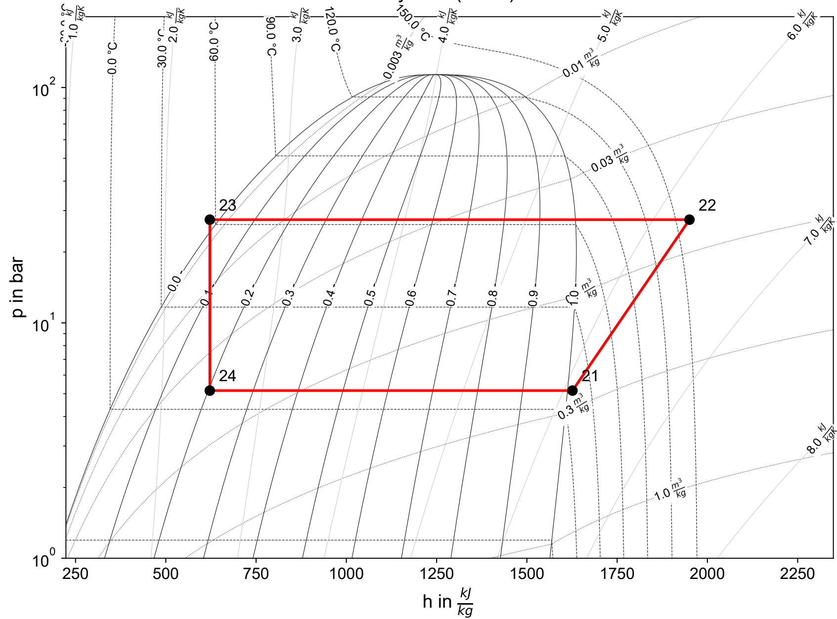
Cycle 1 (R717)
