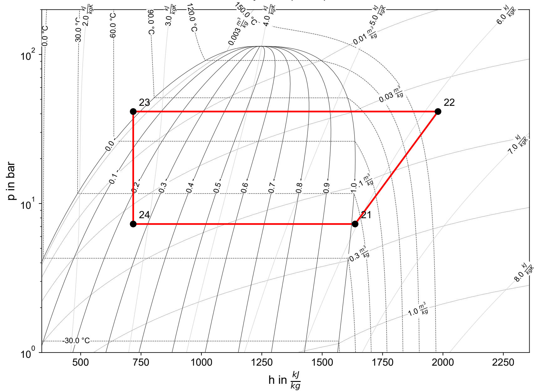
Cycle 1 (R717)
