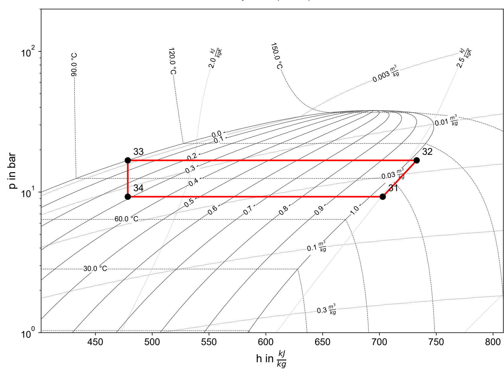
Cycle 2 (R600)
