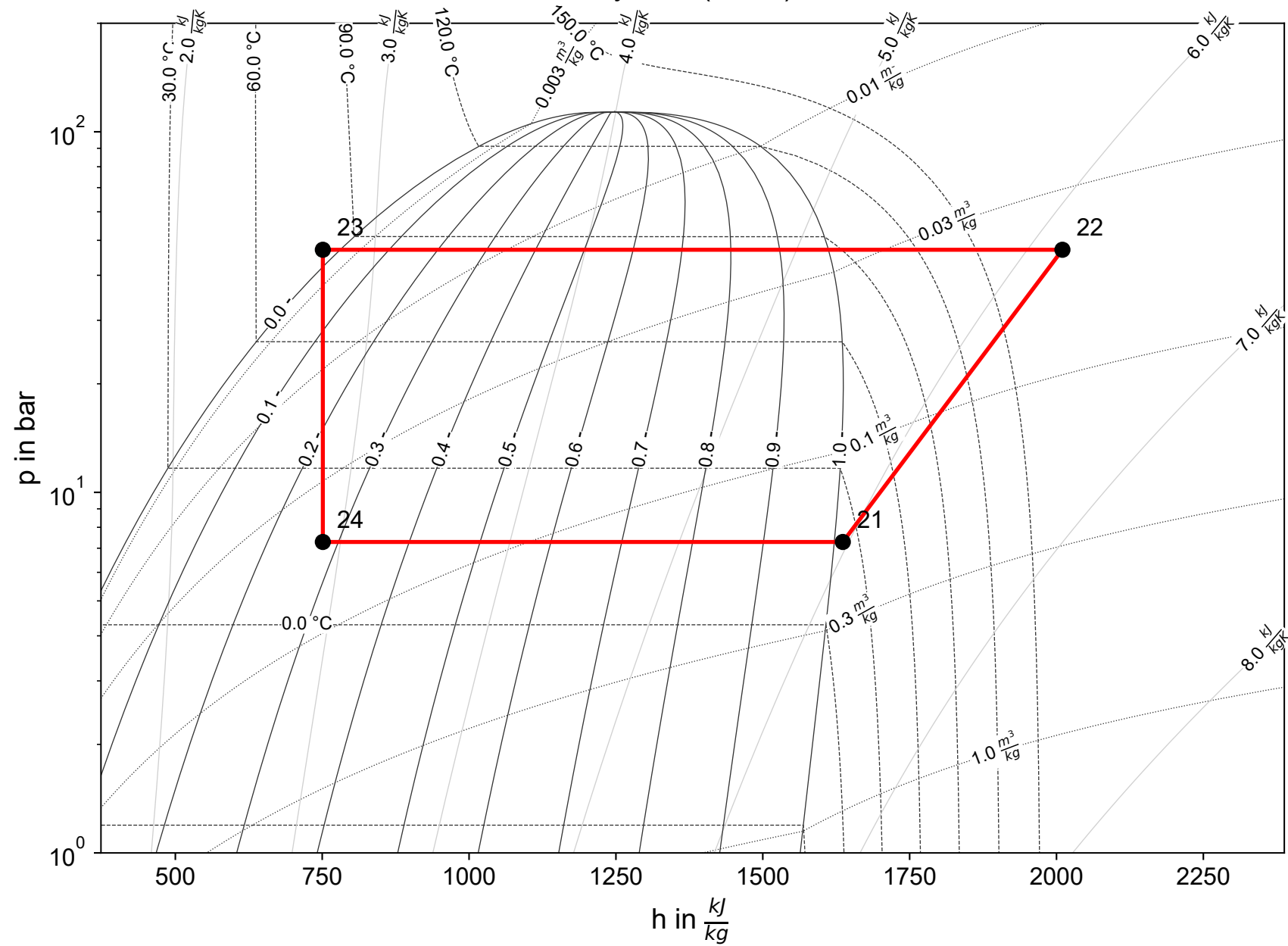
Cycle 1 (R717)
