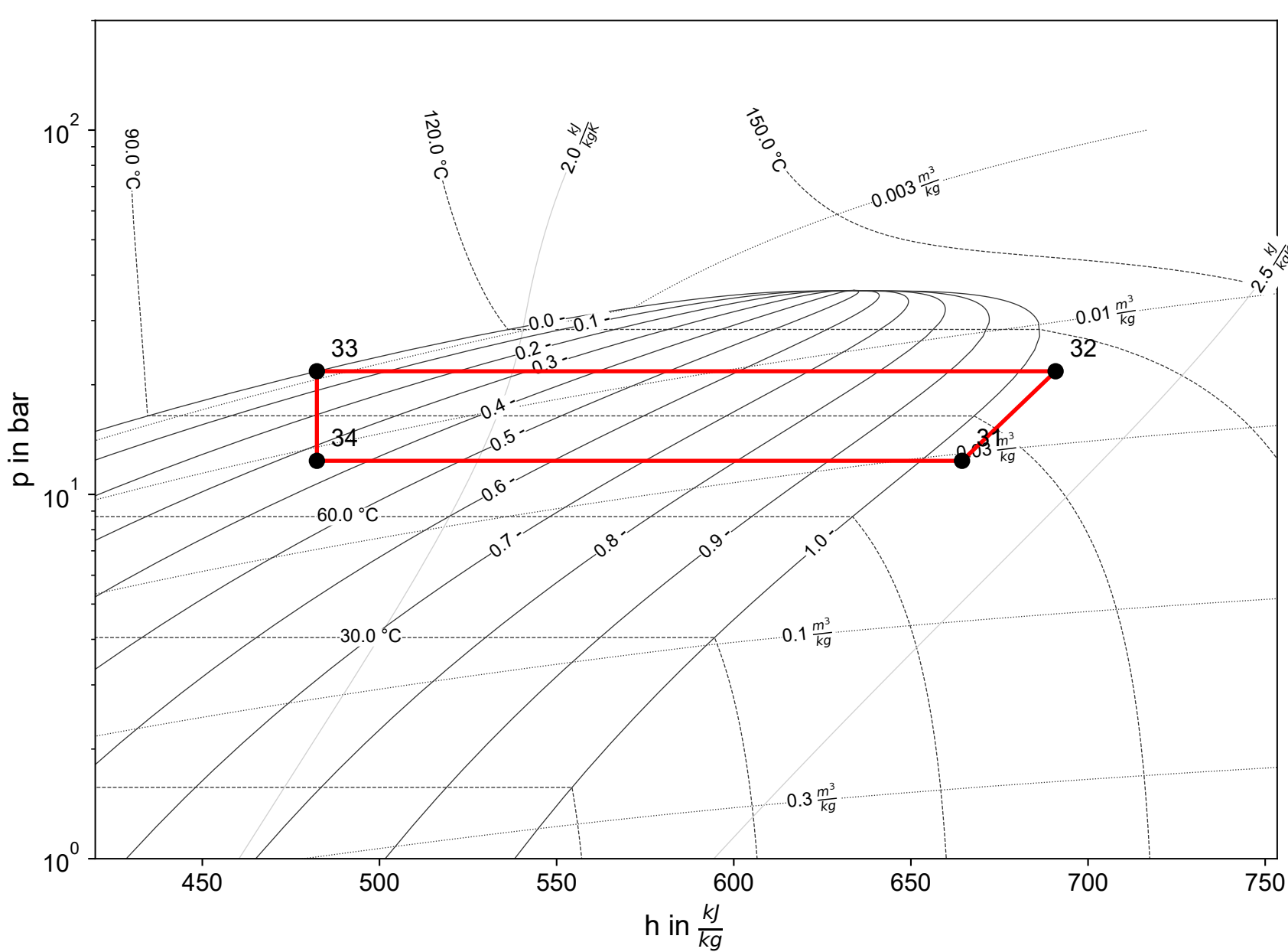
Cycle 2 (R600a)
