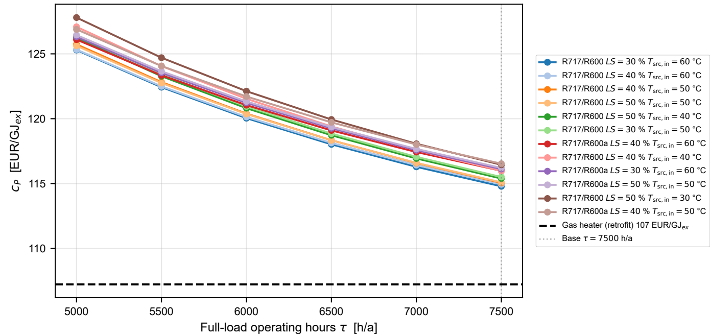
C_P vs full-load hours — 12 cheapest designs ( T_{\text{steam}} = 100\text{ }^{\circ}\text{C} )
