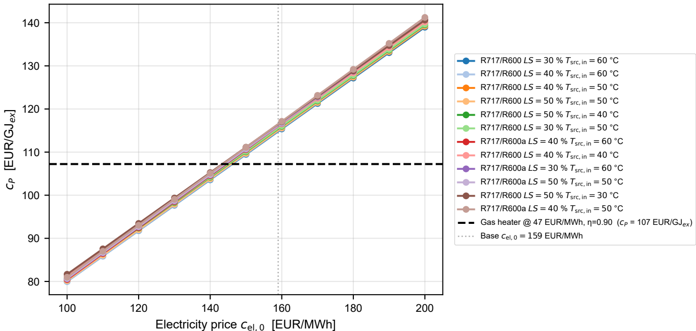
C_p vs electricity price — 12 cheapest designs ( T_{\text{steam}} = 100\text{ °C} )
