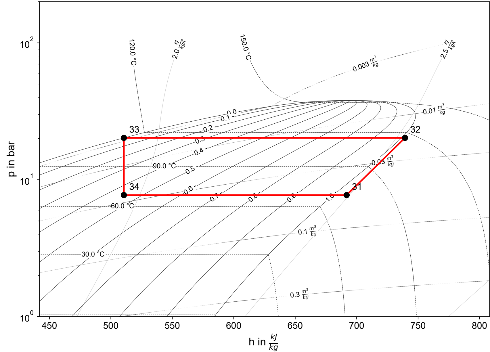
Cycle 2 (R600)
