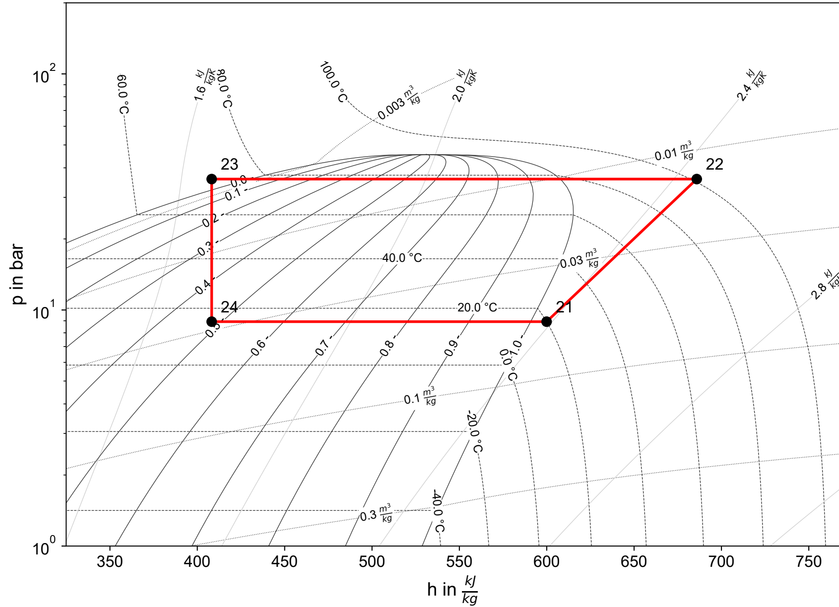
Cycle 1 (R1270)
