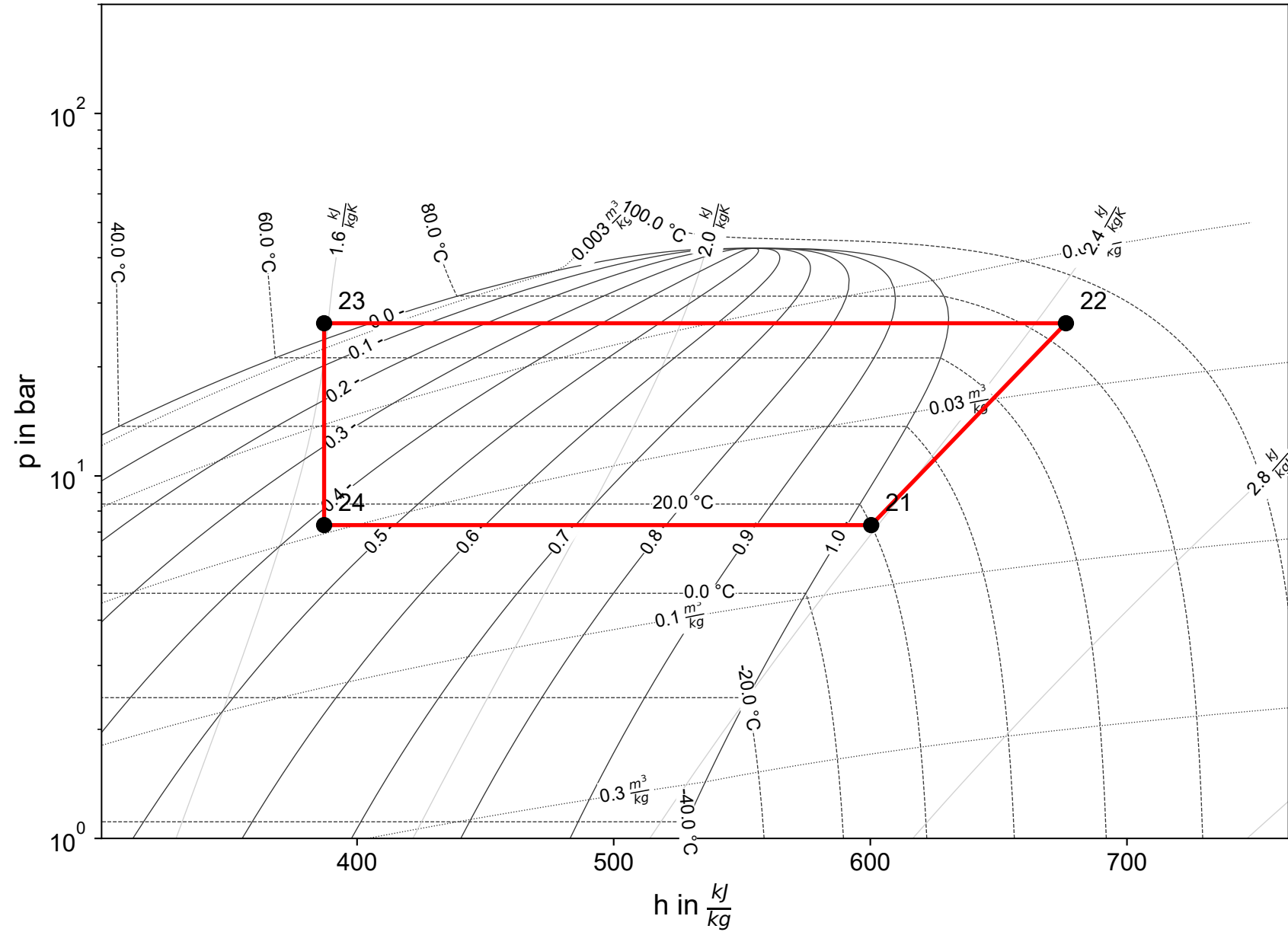
Cycle 1 (R290)
