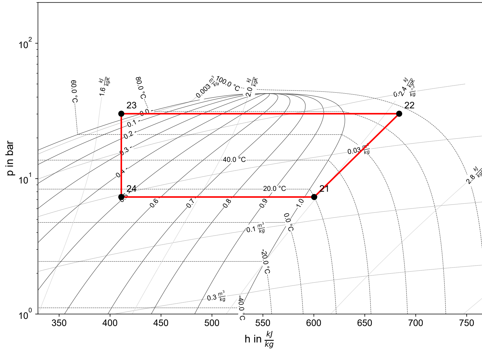
Cycle 1 (R290)
