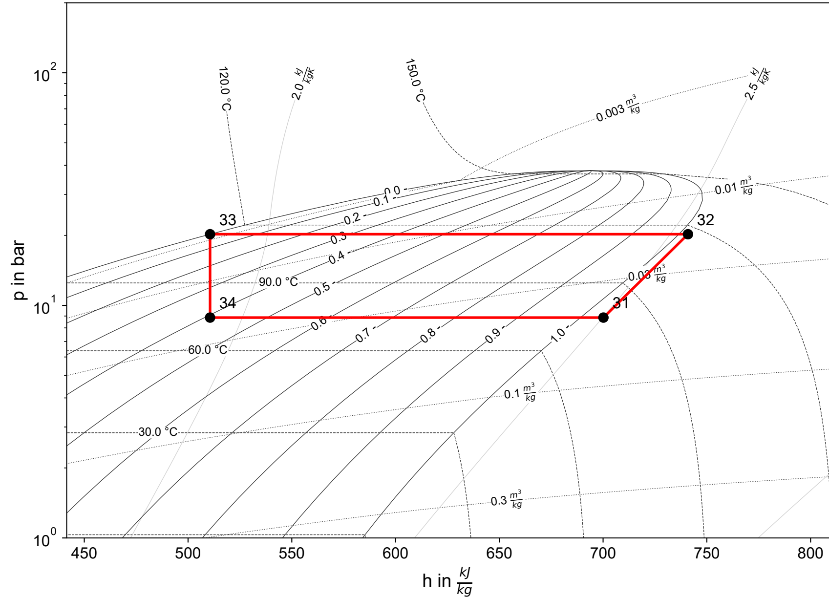
Cycle 2 (R600)
