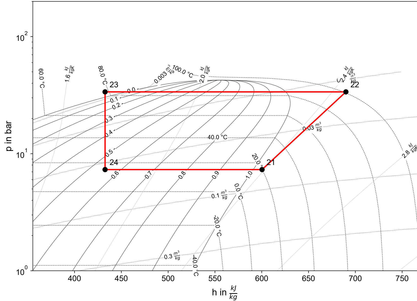
Cycle 1 (R290)
