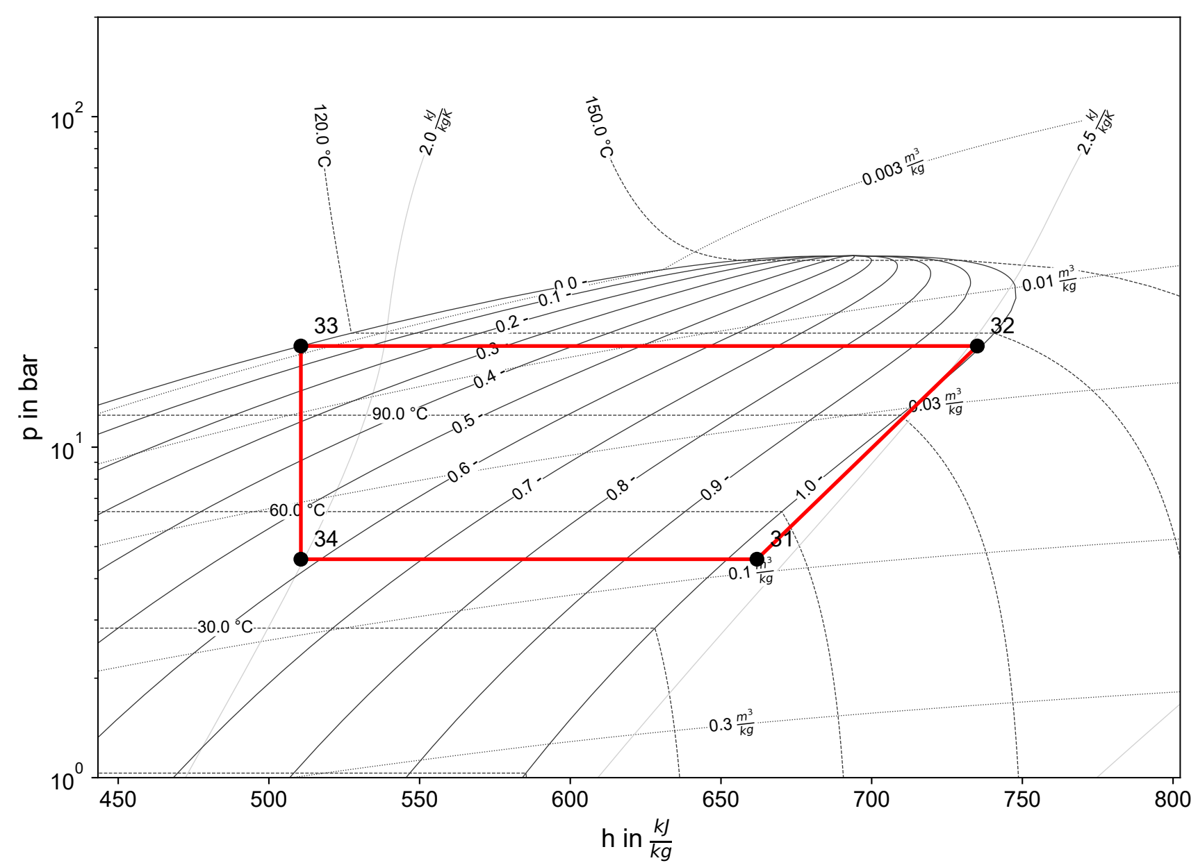
Cycle 2 (R600)
