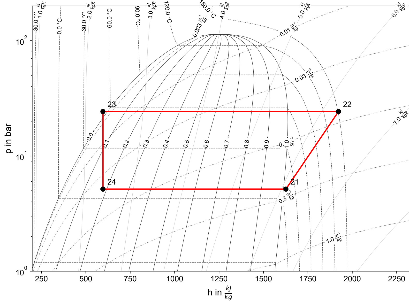
Cycle 1 (R717)
