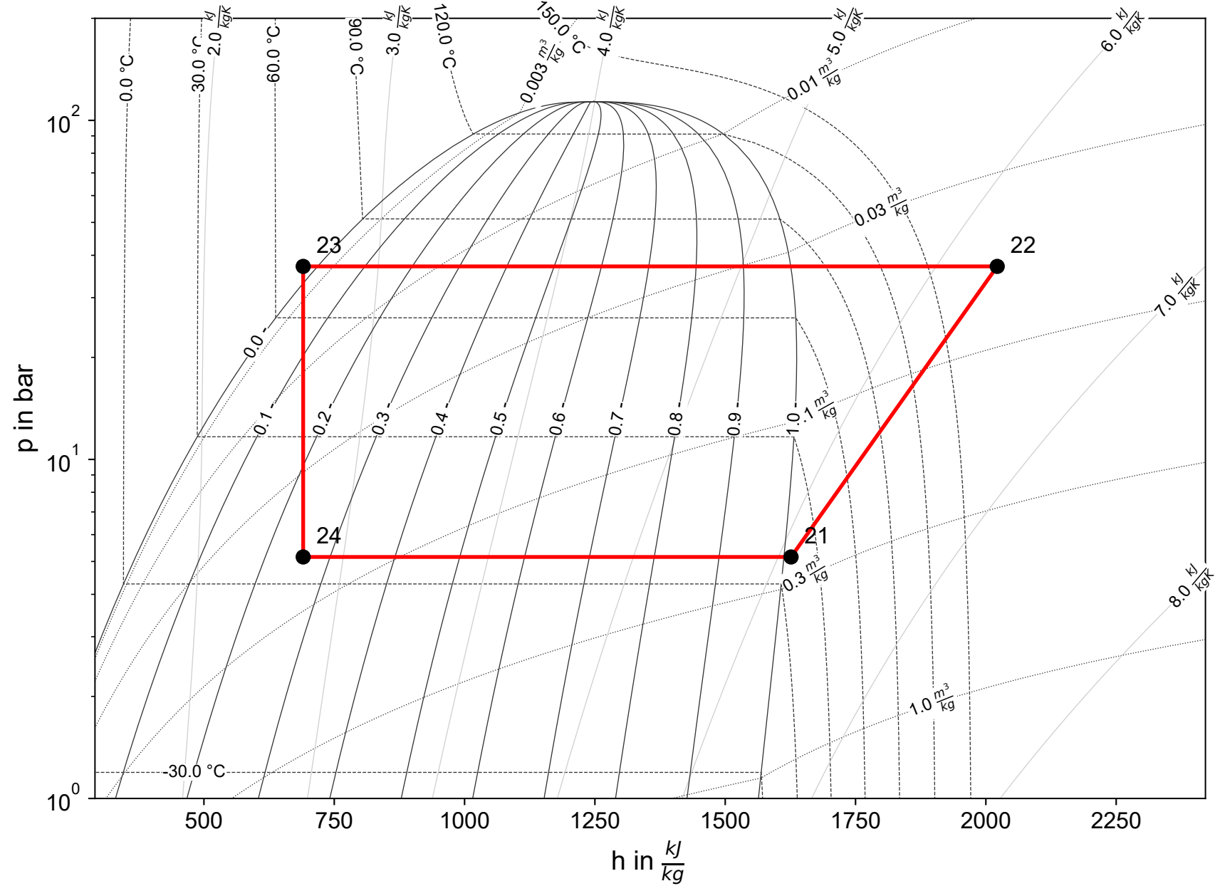
Cycle 1 (R717)
