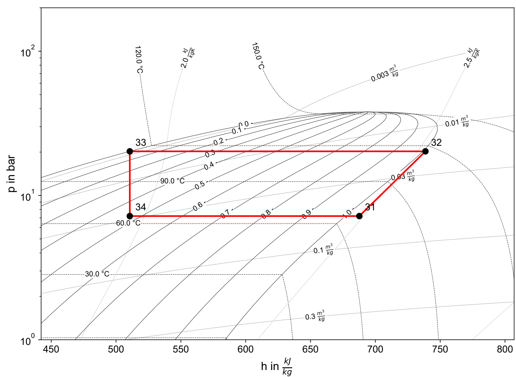
Cycle 2 (R600)
