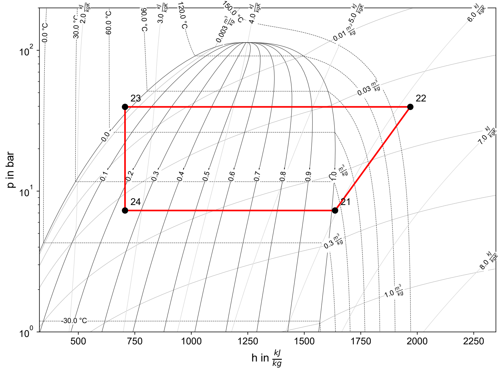
Cycle 1 (R717)
