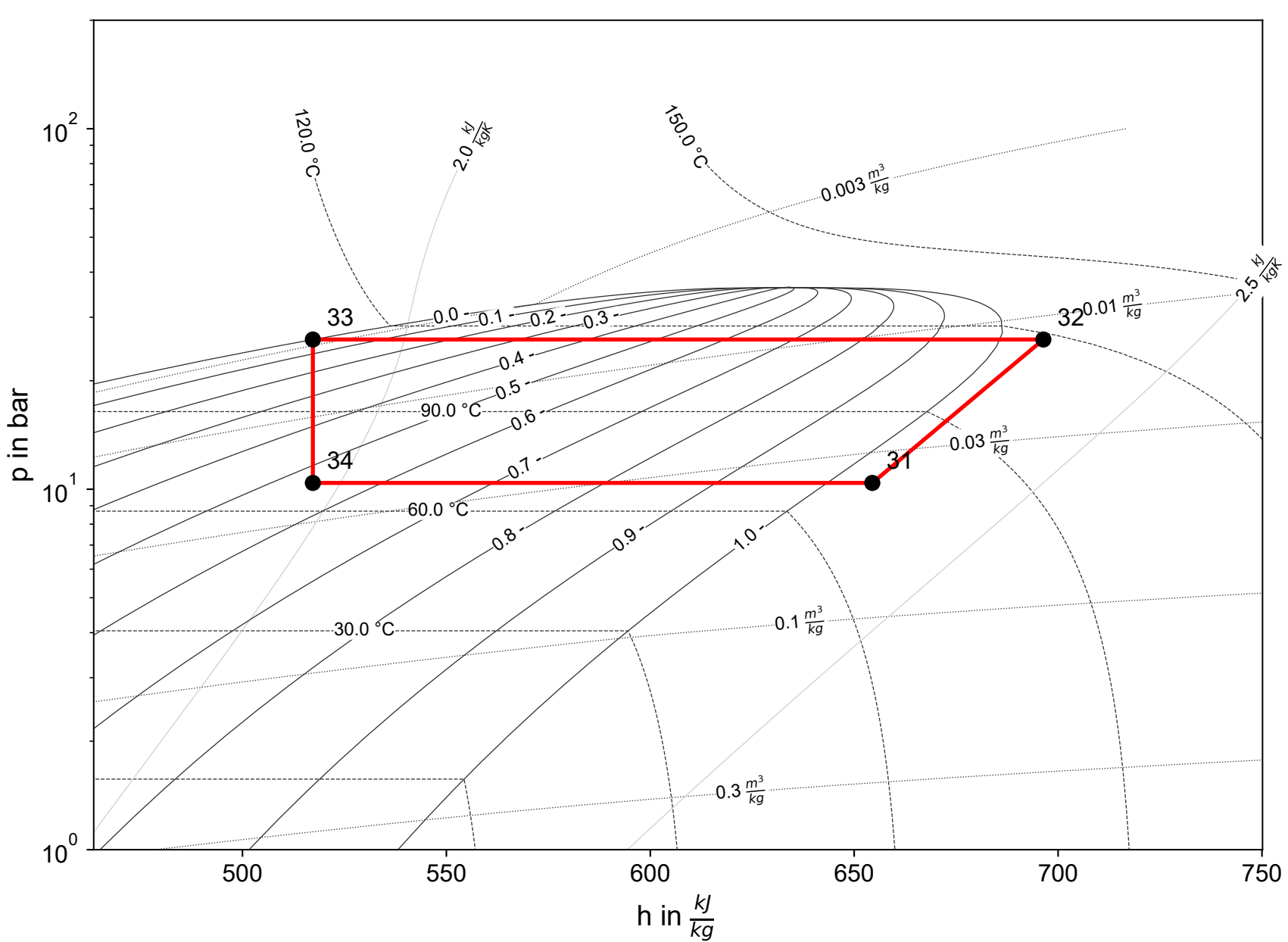
Cycle 2 (R600a)
