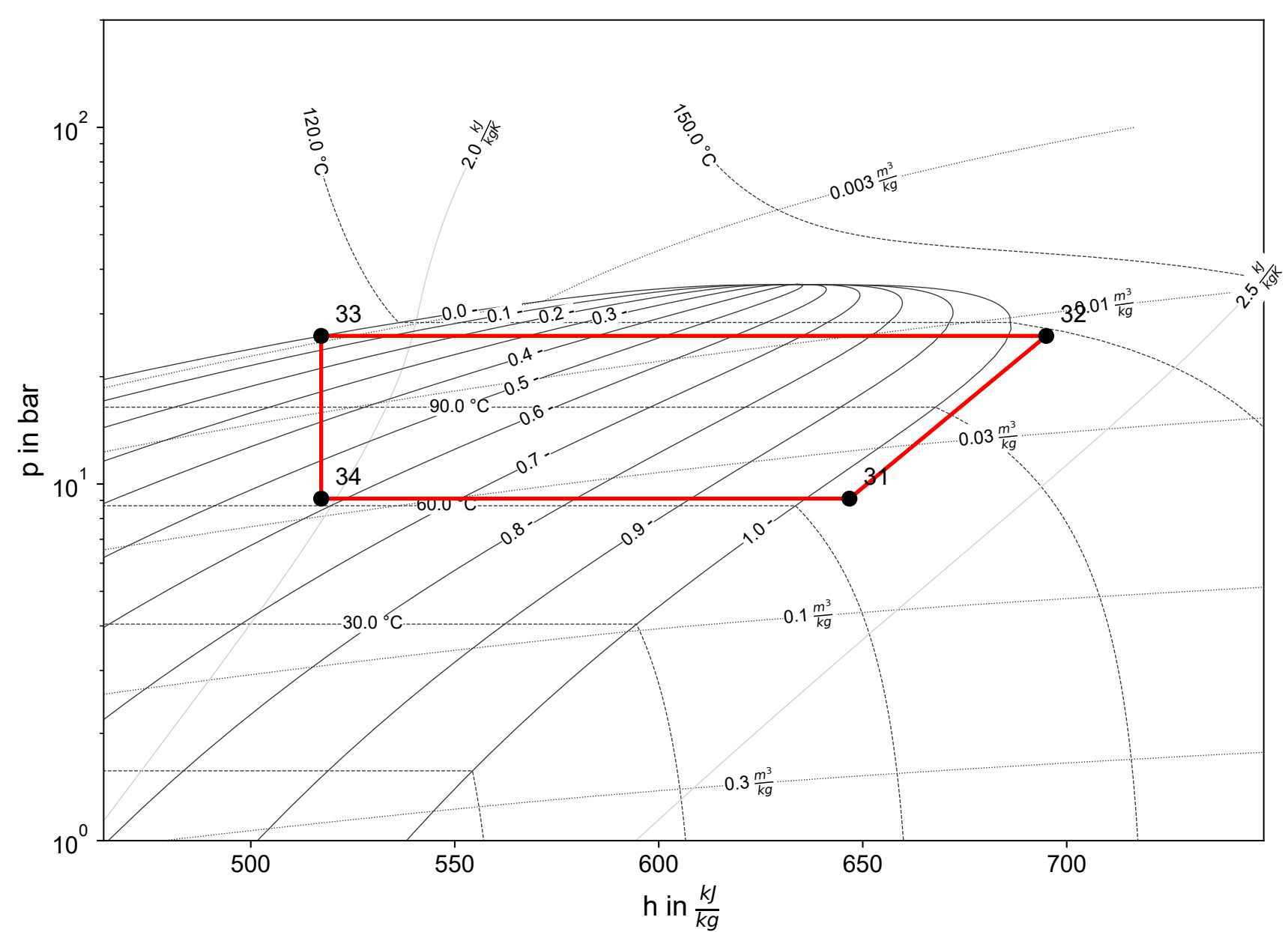
Cycle 2 (R600a)
